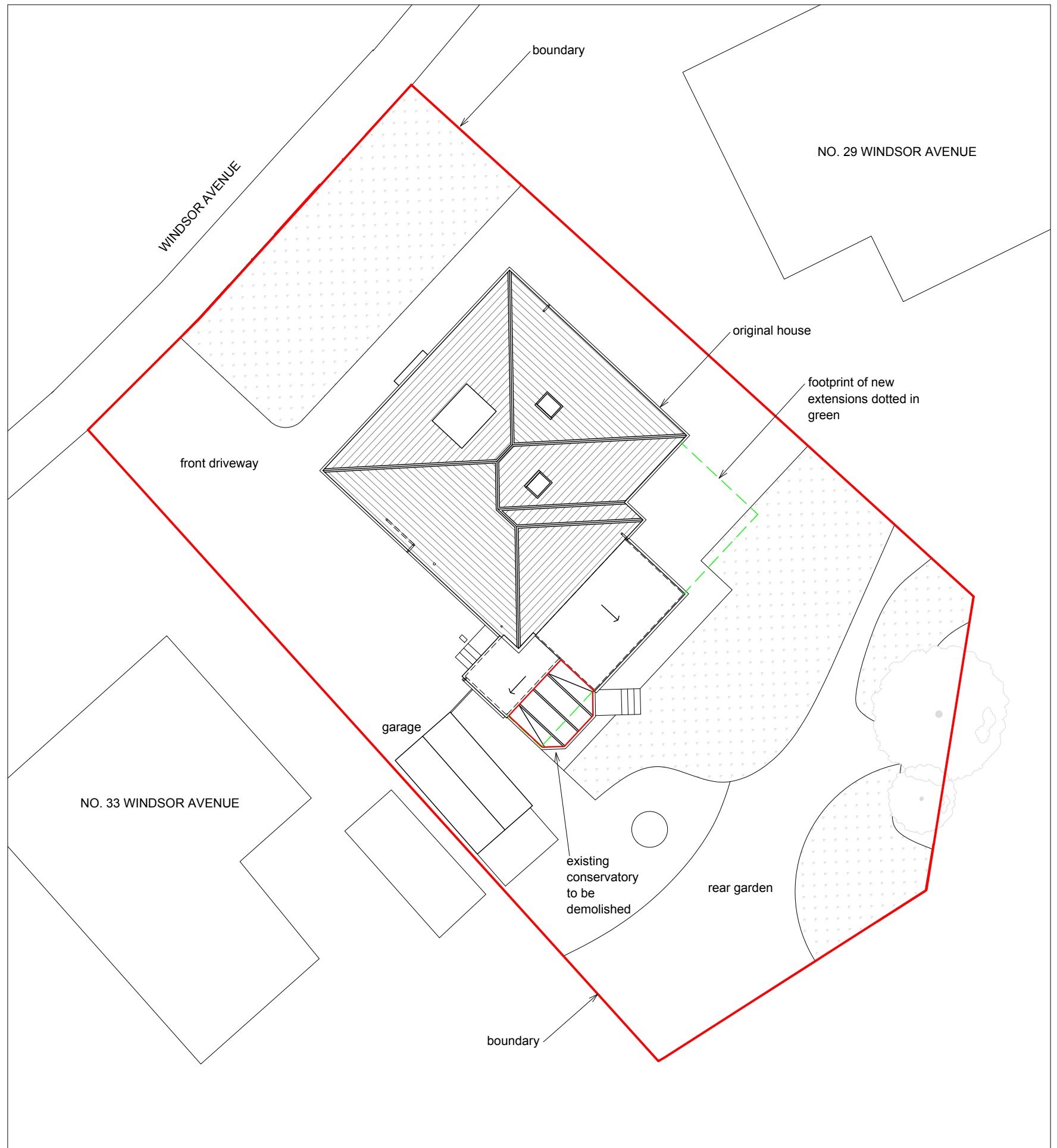
BLOCK PLAN 1:200
