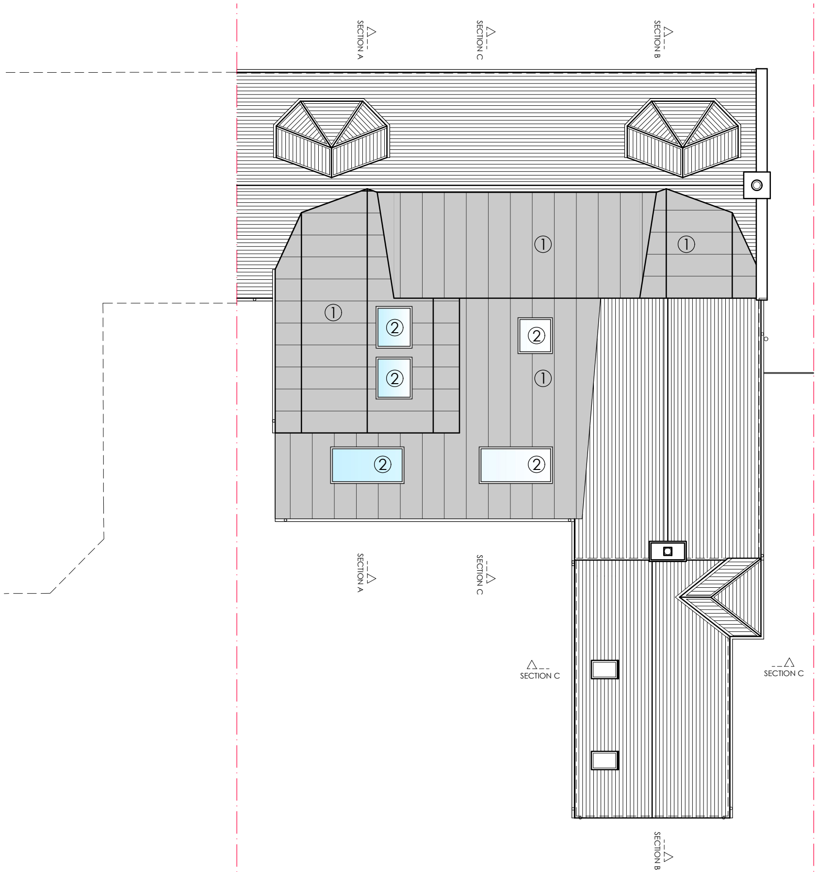
ROOF PLAN AS PROPOSED
