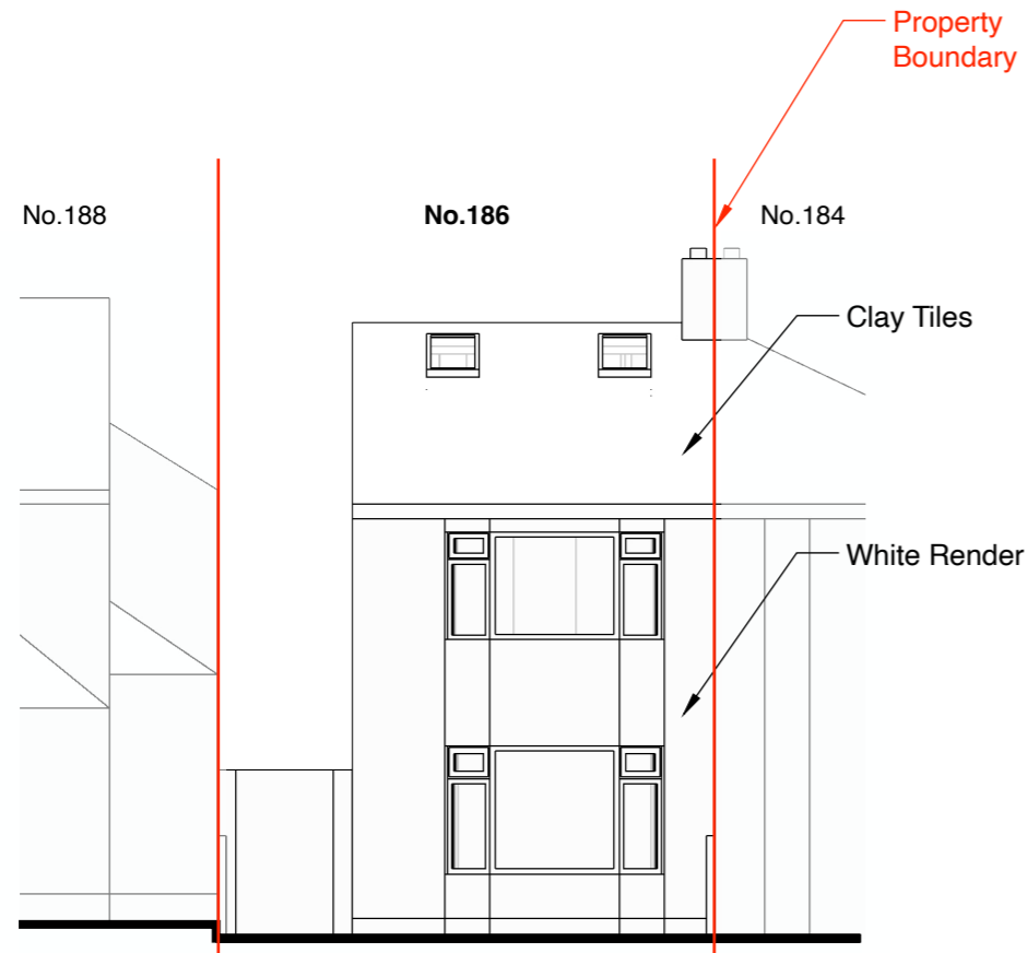
1 Street Elevation - Existing
