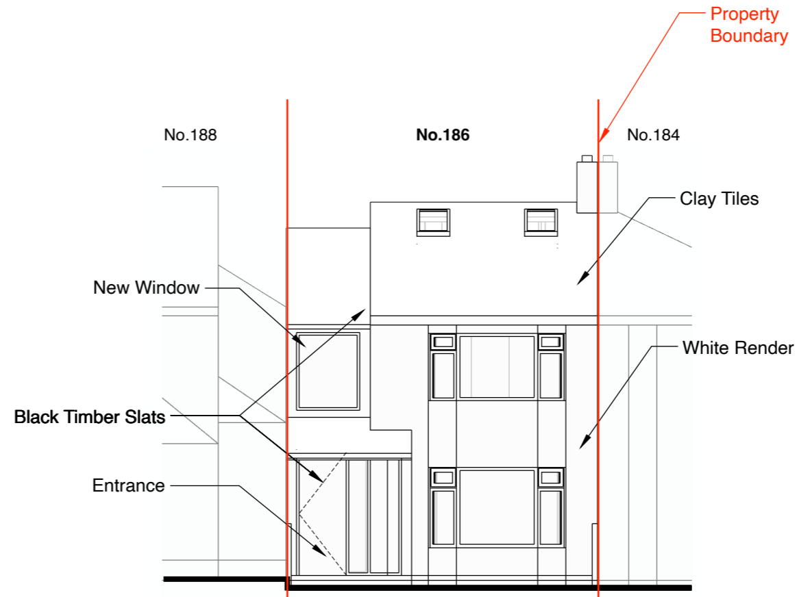
2 Street Elevation - Proposed
