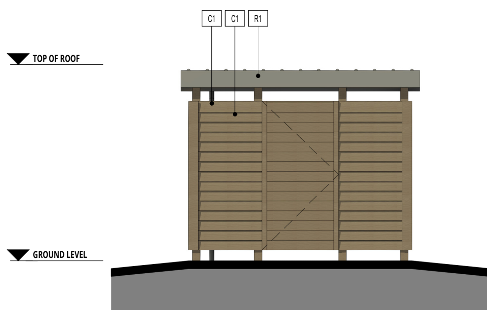
ELEVATION C
