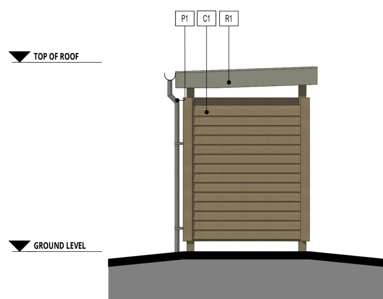
ELEVATION D
