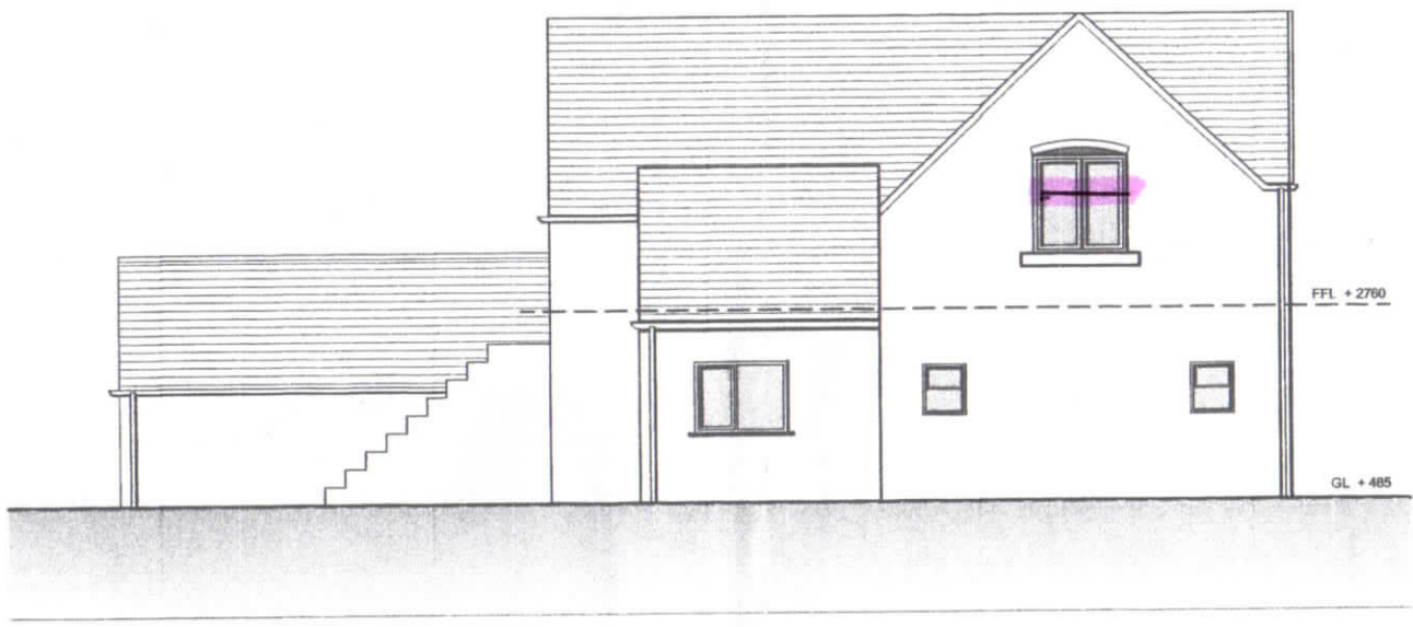
Side Elevation
