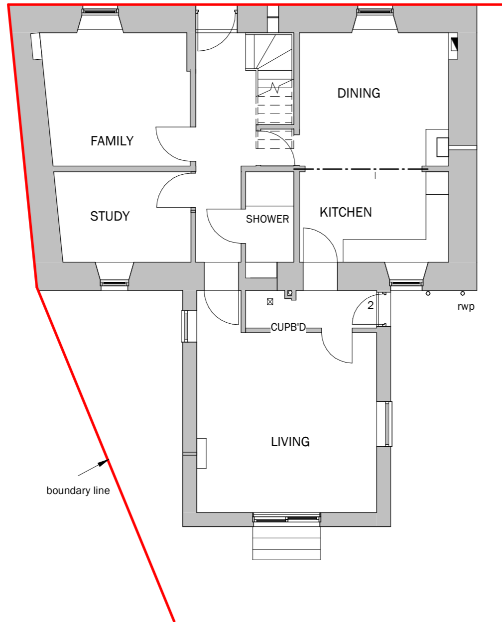
Ground Floor - Existing 1 : 100
