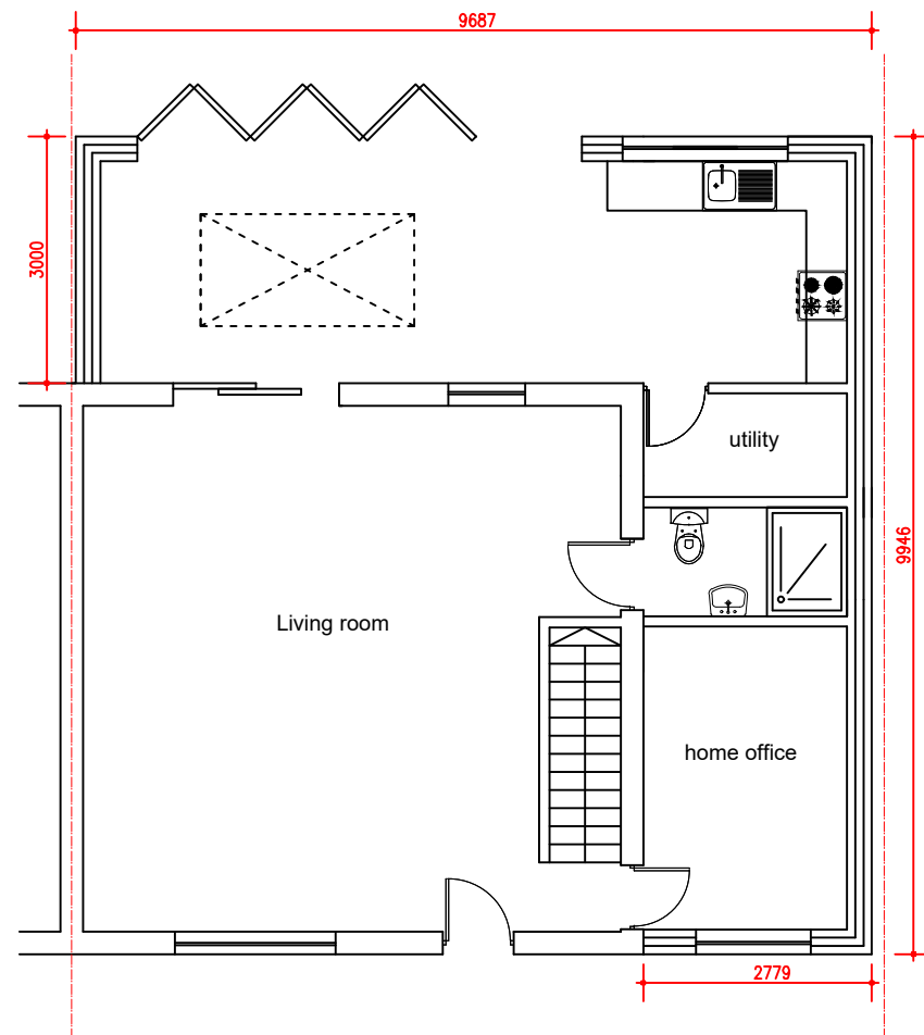
APPROVED GROUND FLOOR PLAN
