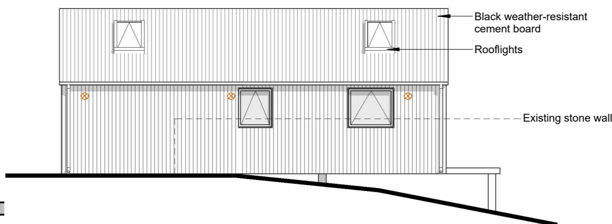
Front Elevation - Lighting Arrangement
