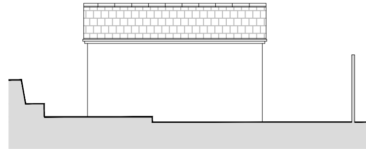
South East Elevation 1 : 100 @ A3
