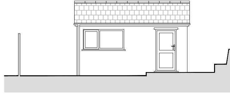
North West Elevation 1 : 100 @ A3
