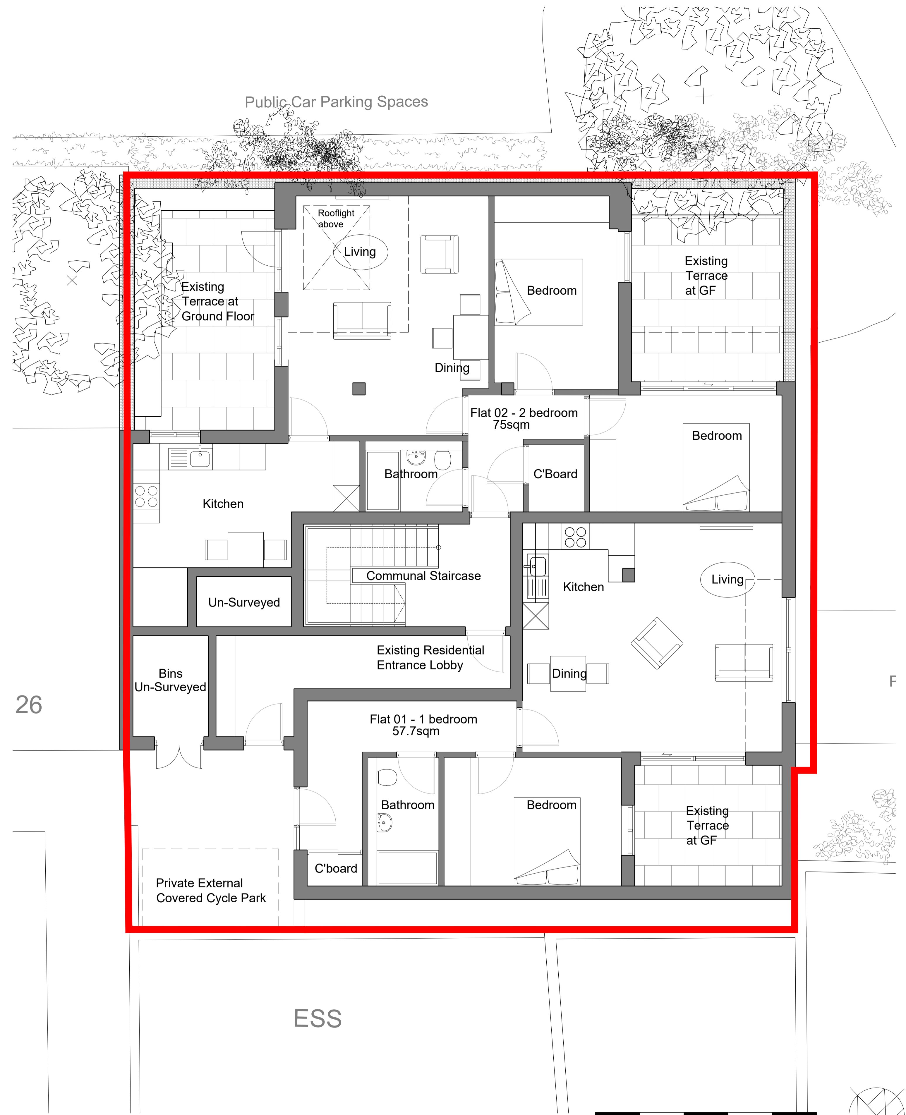
01 Ground Floor Plan: Proposed
