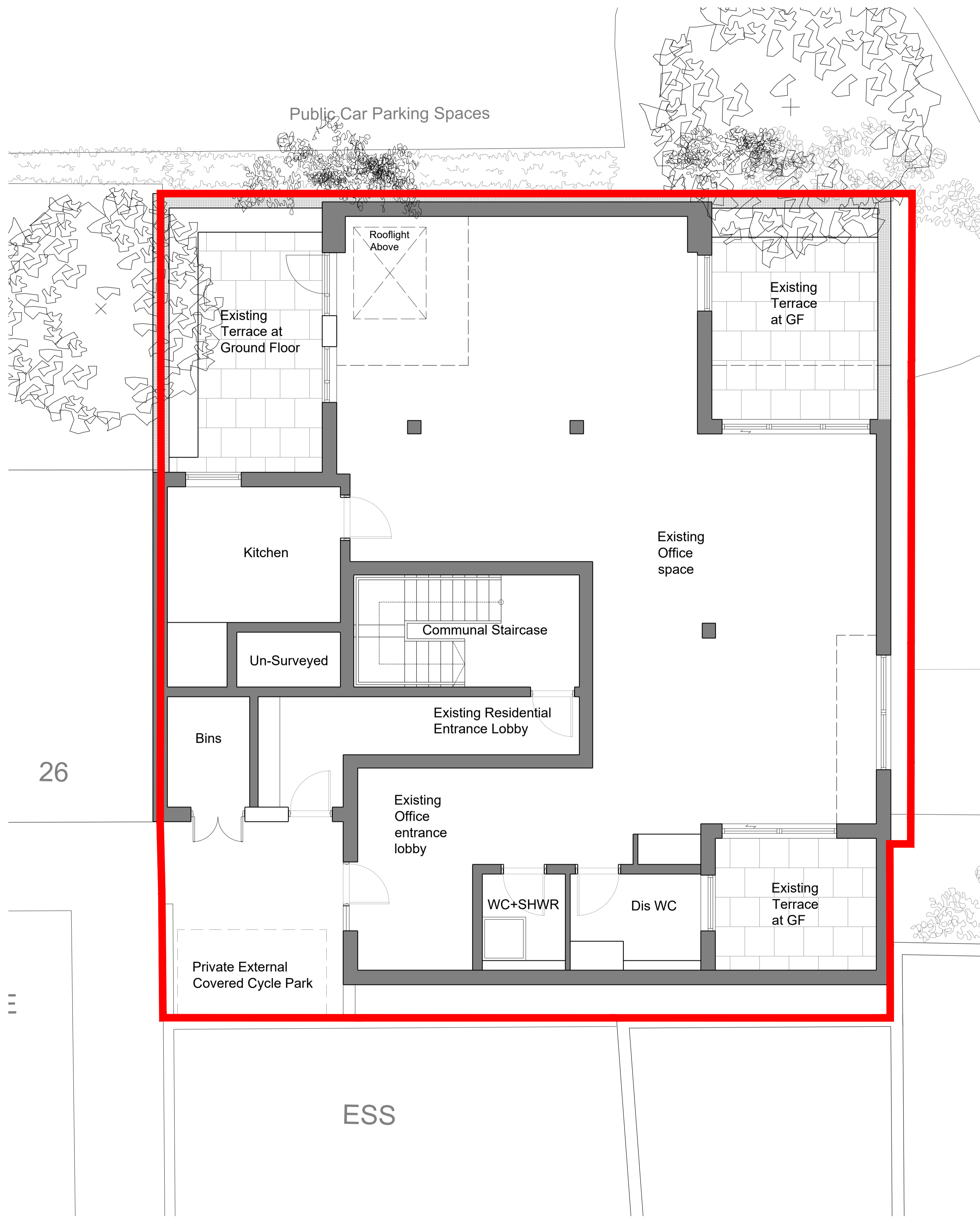
00 Ground Floor Plan: Existing
