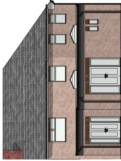
Proposed Rear Elevation 1:100
