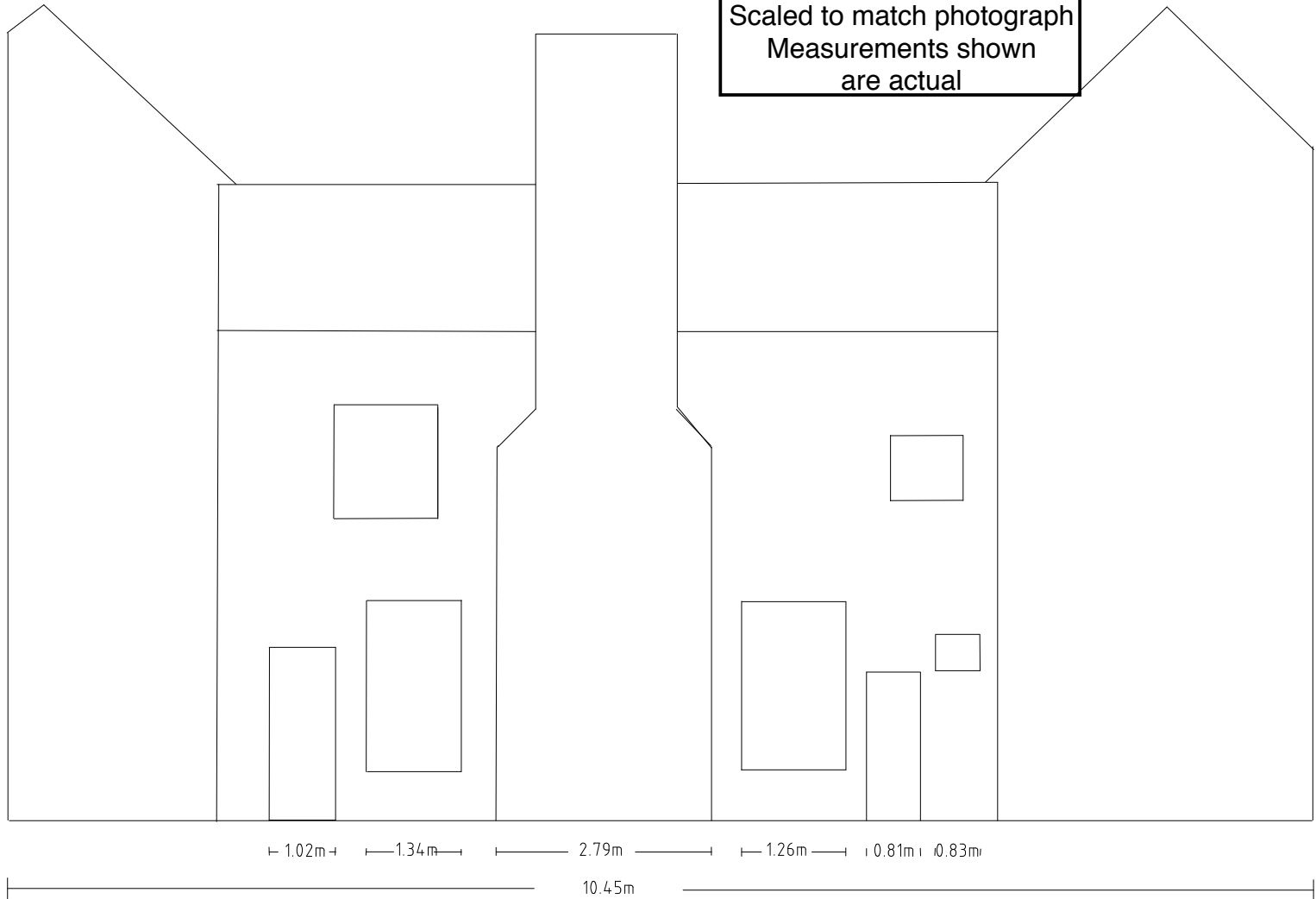
LBH Rear Elevation
