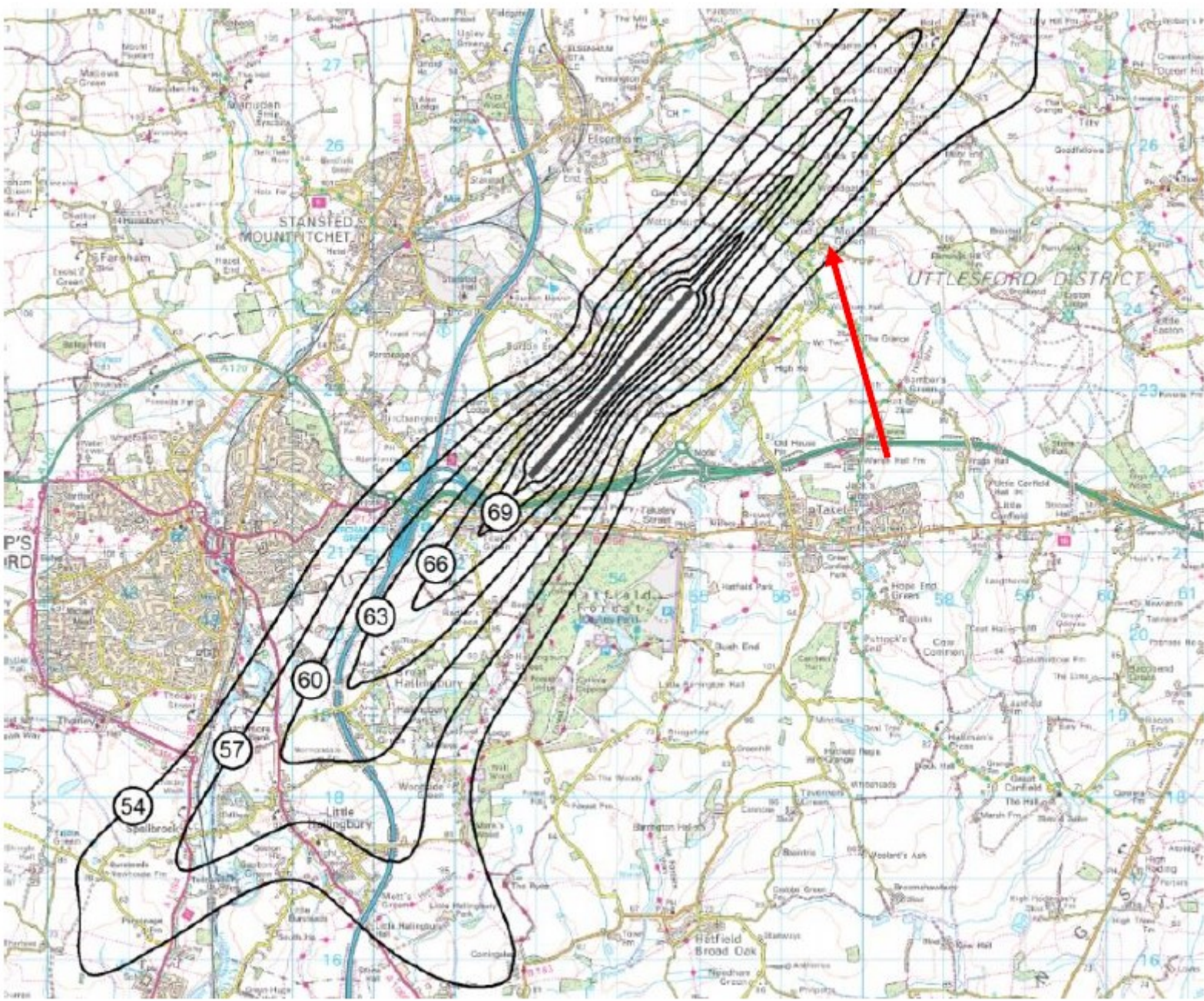
NOISE EXPOSURE CONTOURS FOR STANSTED AIRPORT 2017
