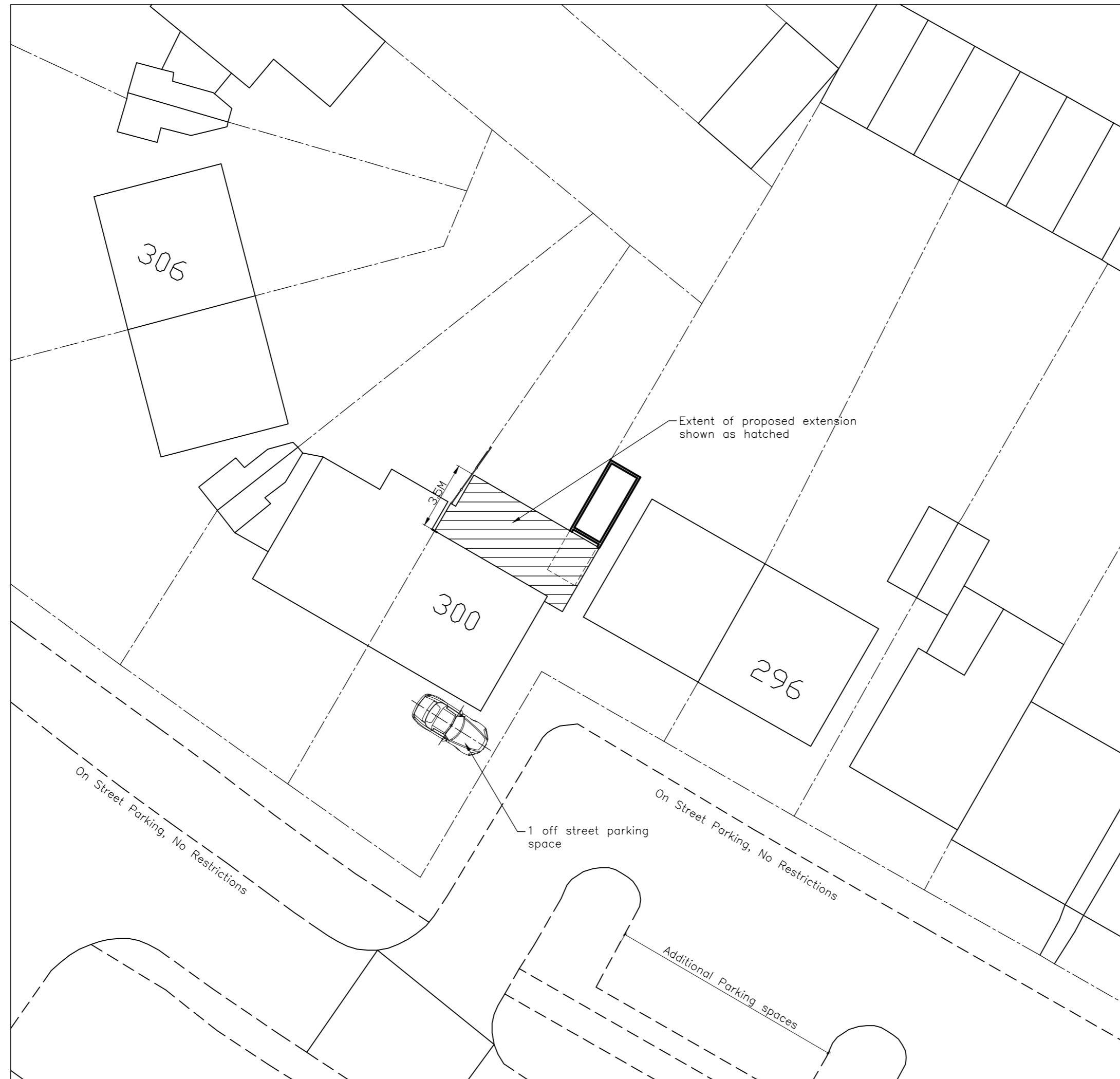
BLOCK PLAN (1:200)
