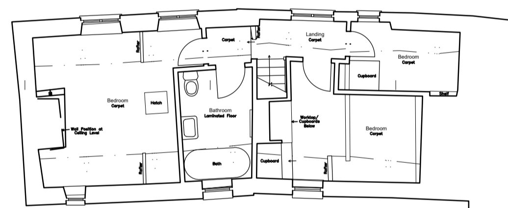
FIRST FLOOR PLAN 1:100
