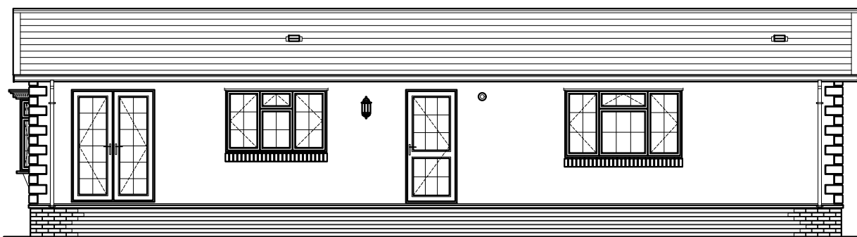
Nearside Elevation
