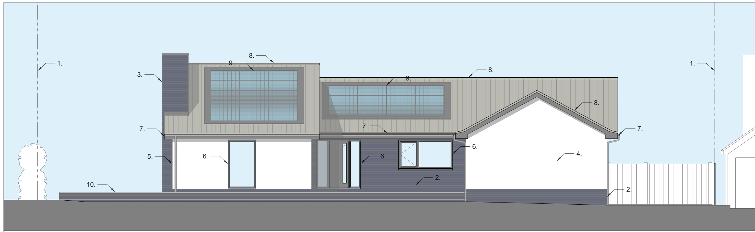
PROPOSED SOUTH ELEVATION 0 1 2
