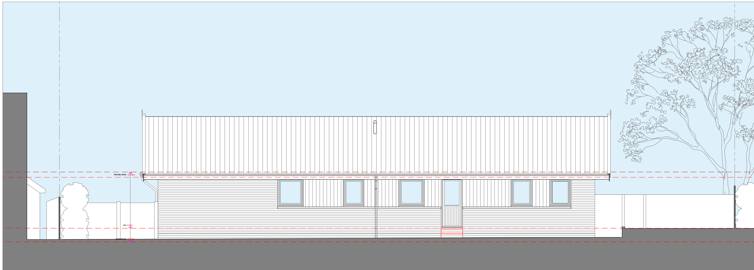
EXISTING NORTH ELEVATION 0 1 2
