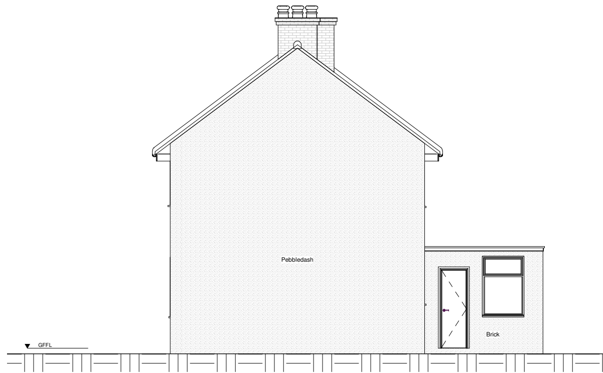
1 Existing East (Right) 1 : 100
