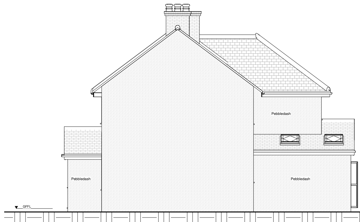
3 Proposed East (Right) 1 : 100
