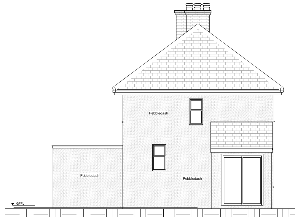
2 Existing West (Left) 1 : 100
