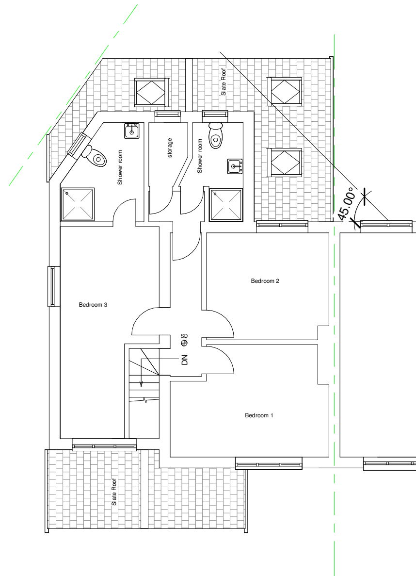
② Proposed First Floor 1 : 100
