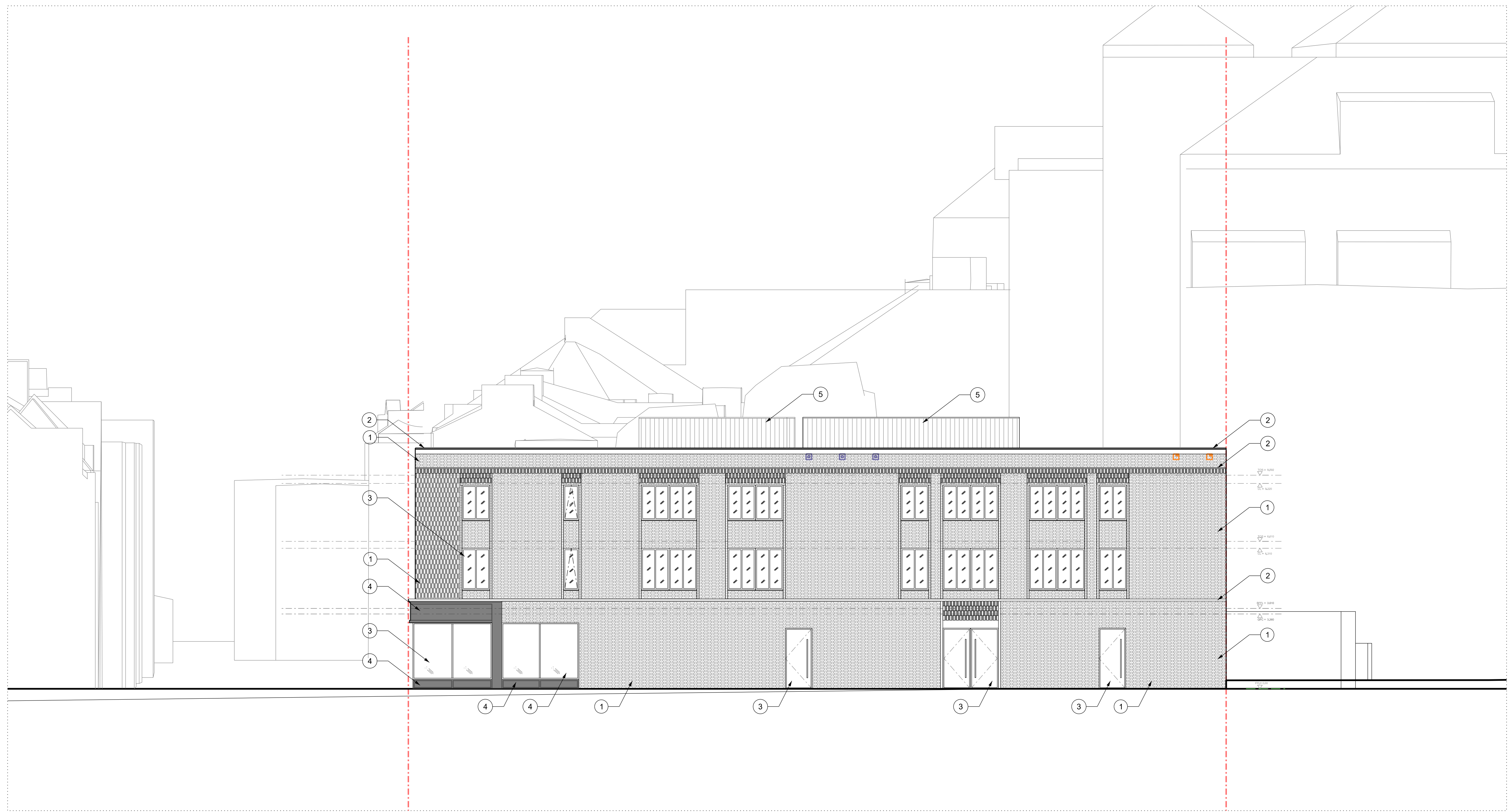
Proposed North Elevation
