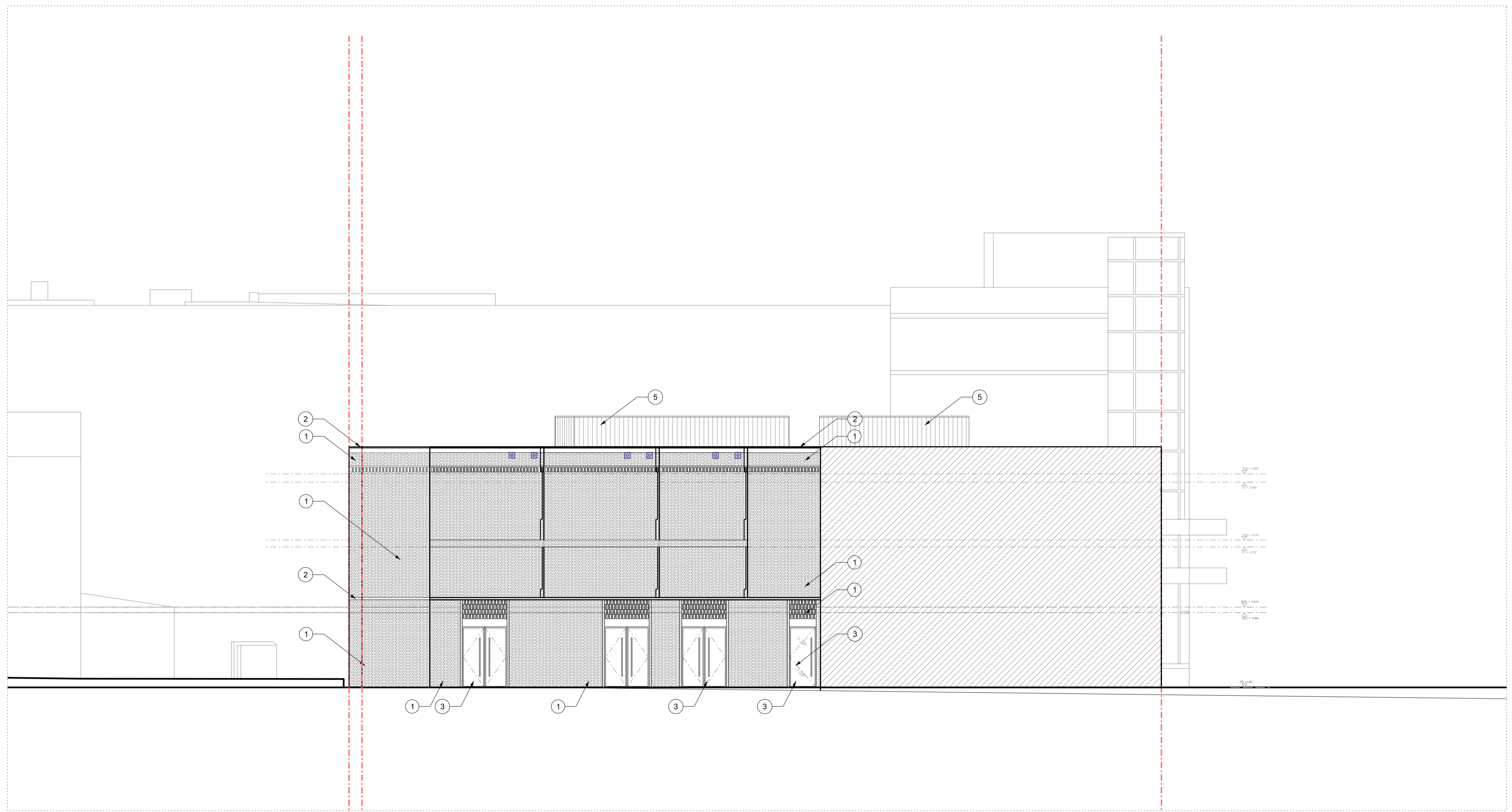
Proposed South Elevation
