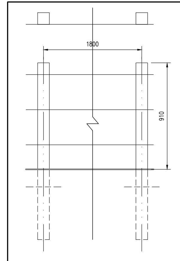
EXISTING FENCE DETAIL Scale 1:20
