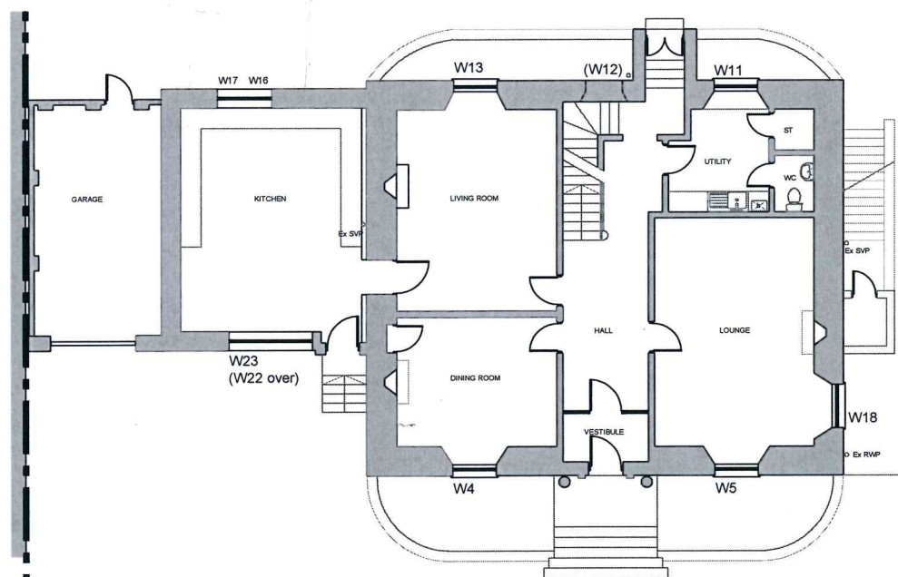
Ground Floor Plan as Existing 1:100
