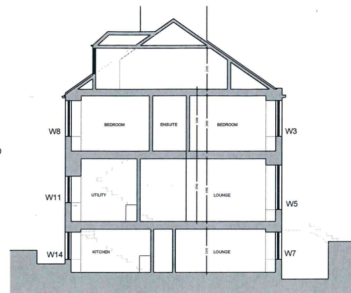
Section as Existing 1:100
