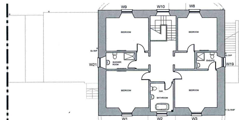
First Floor Plan as Existing 1:100
