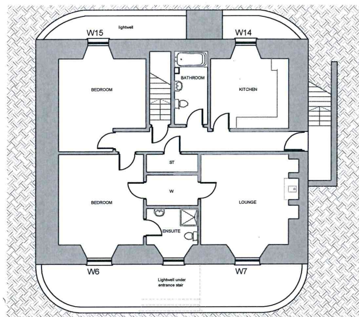
Basement Floor Plan as Existing 1:100
