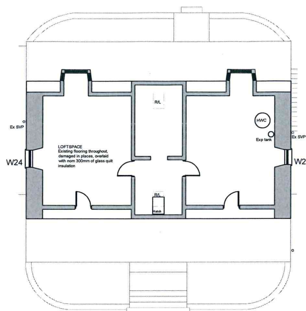
Second Floor Plan as Existing 1:100
