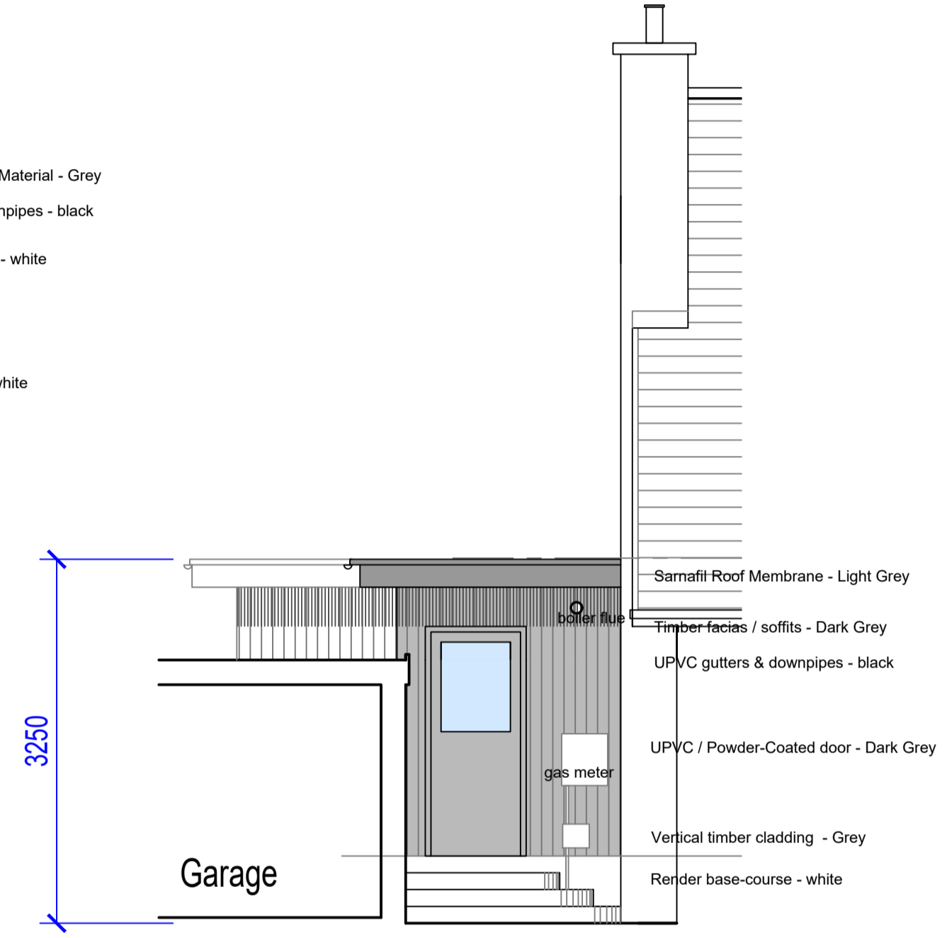
Hidden Front (West) Elevation as Proposed 1:50
