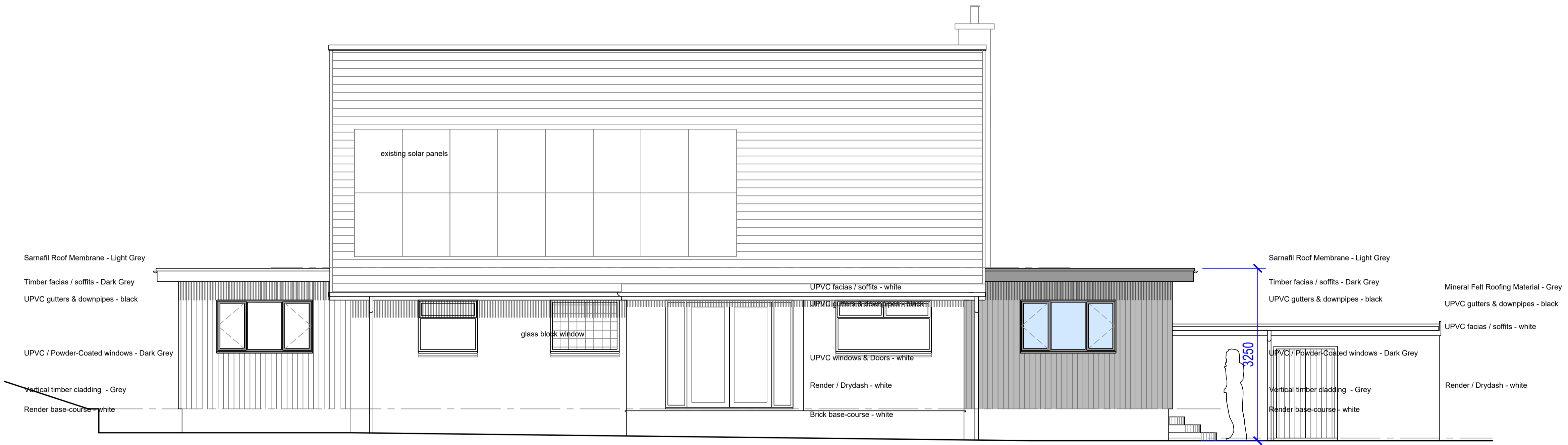
Rear (East) Elevation as Proposed 1:50
