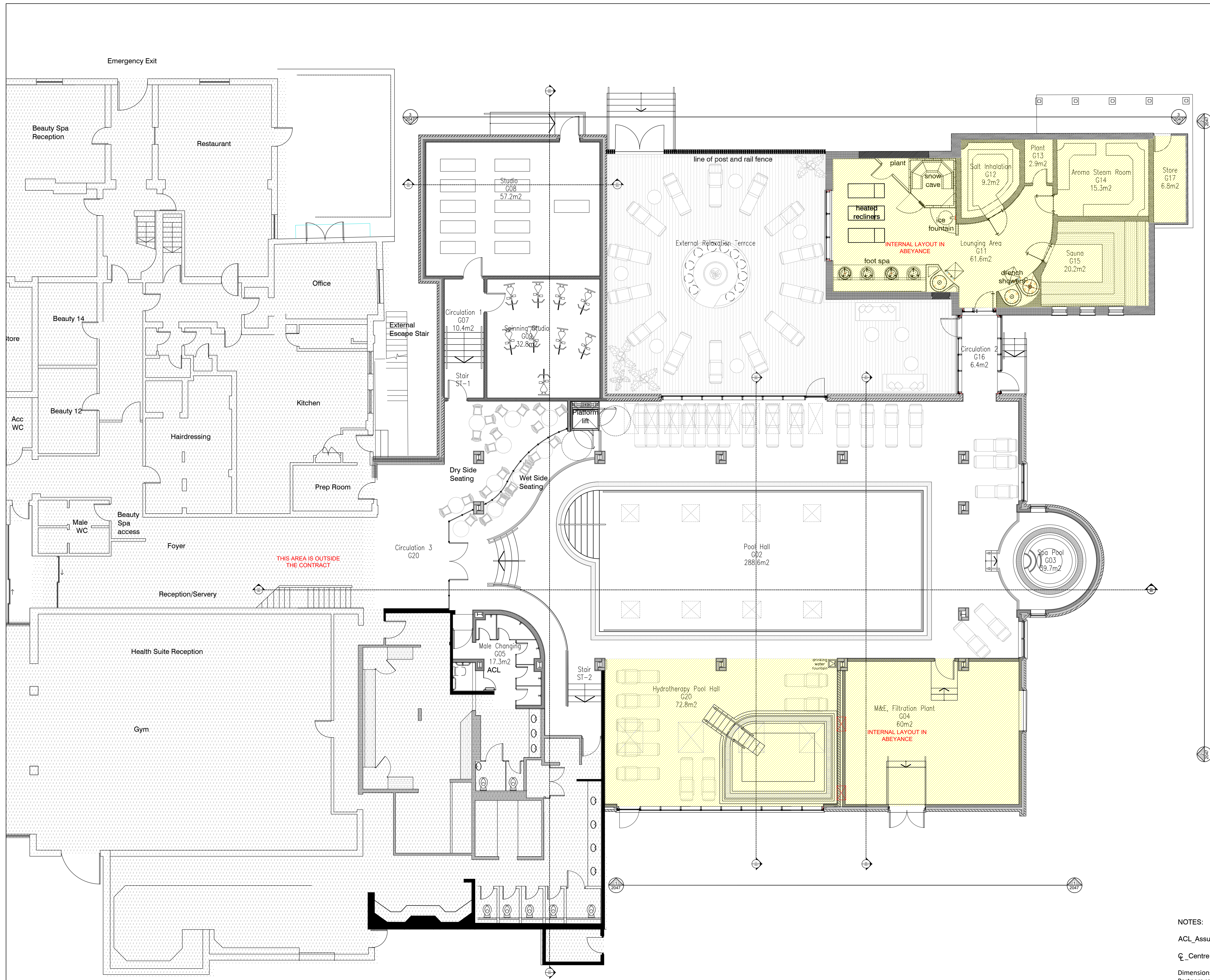
GROUND FLOOR PLAN SCALE 1:100
