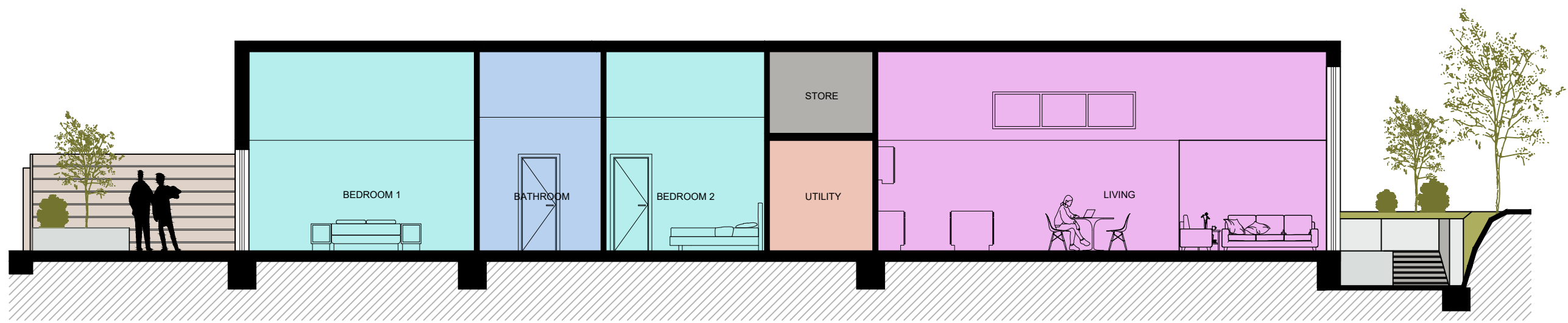
Section BB
