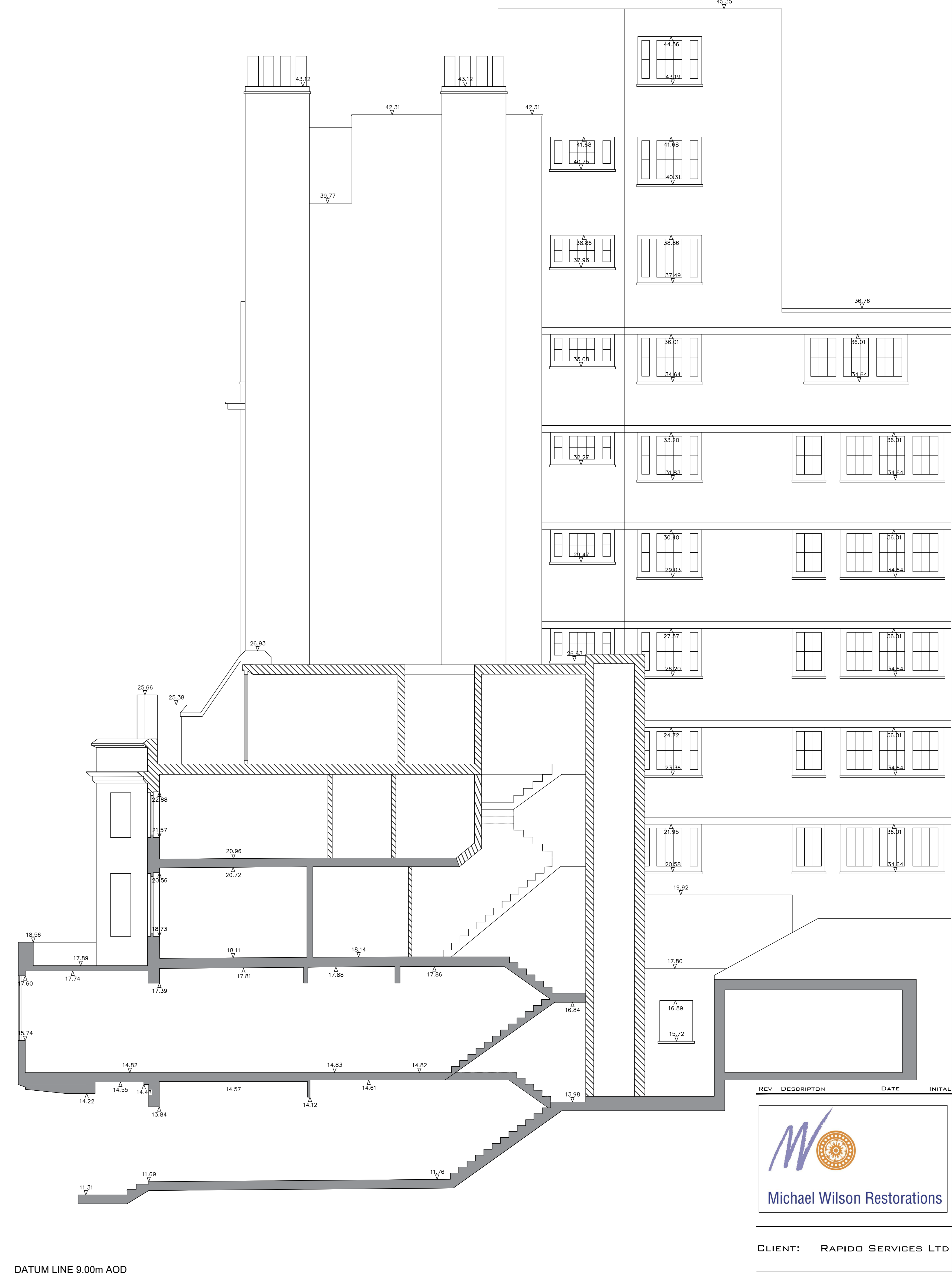
SECTION BB
