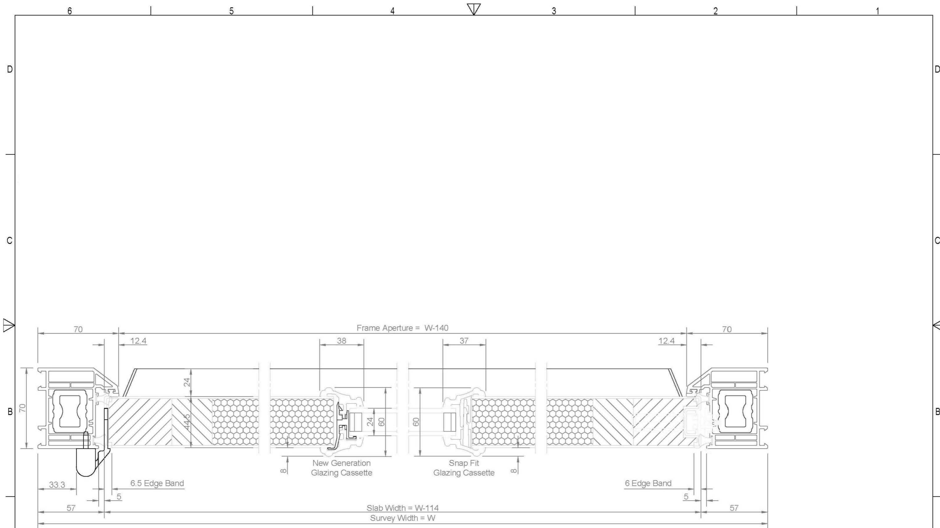
Open-In Door
