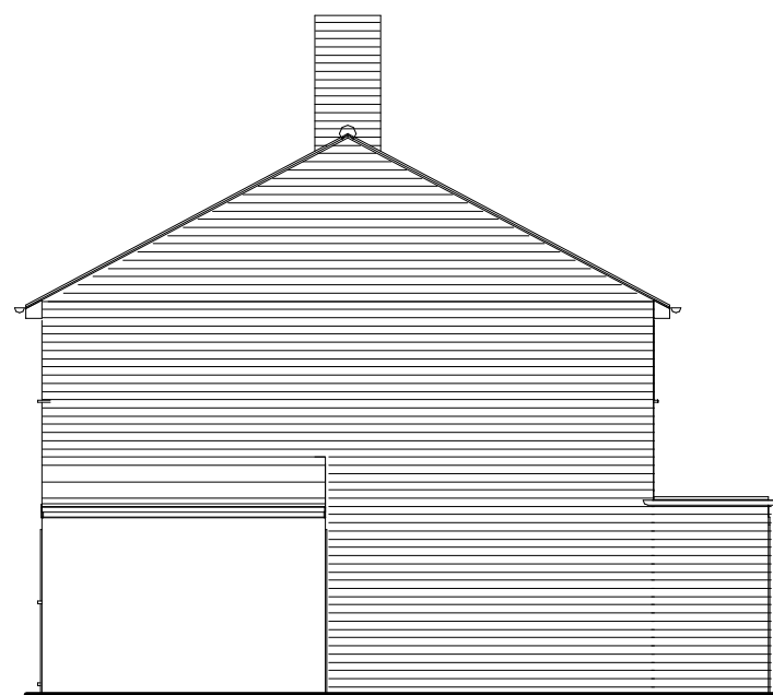
EXISTING LH SIDE ELEVATION
