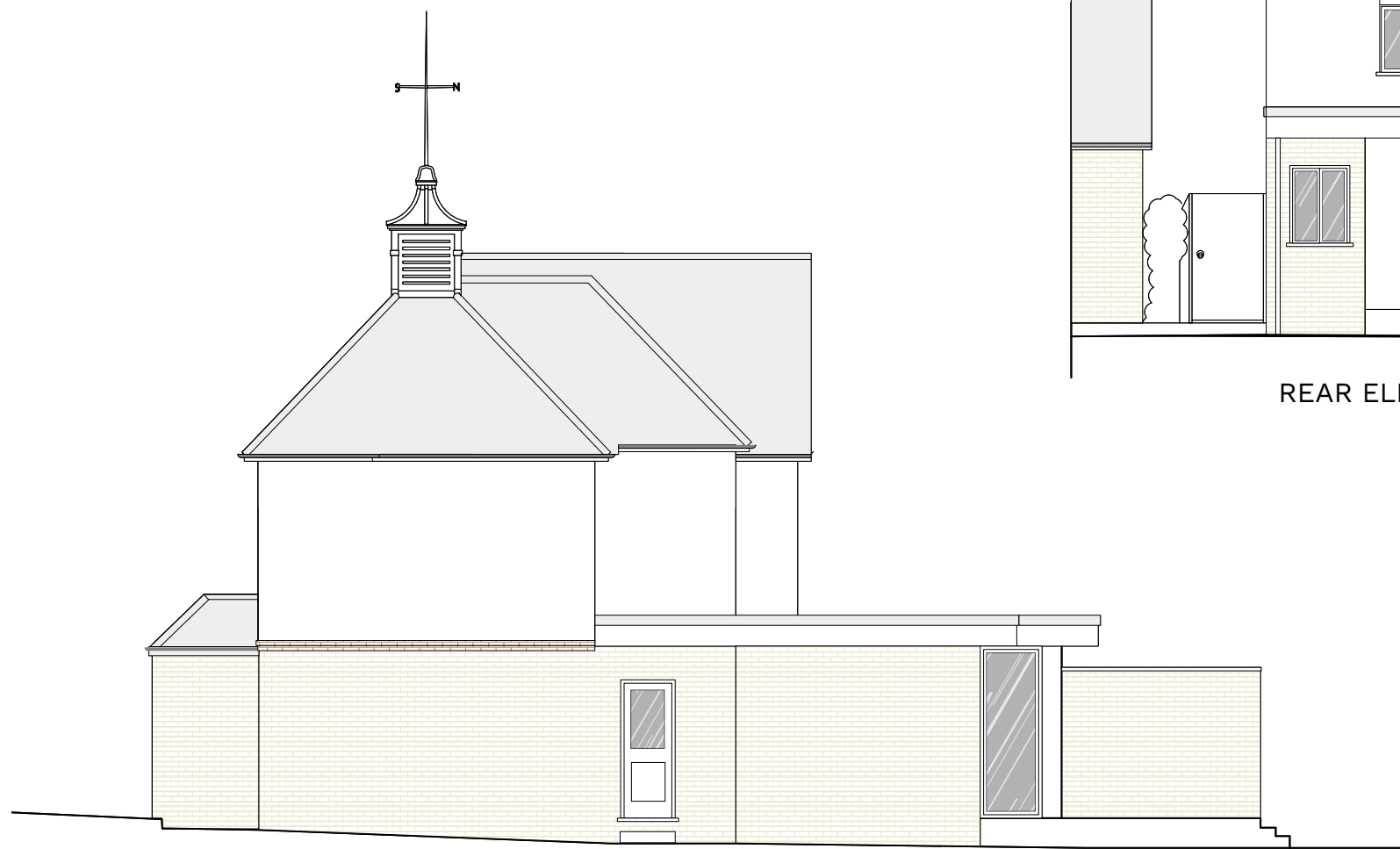
SIDE ELEVATION (SW)
