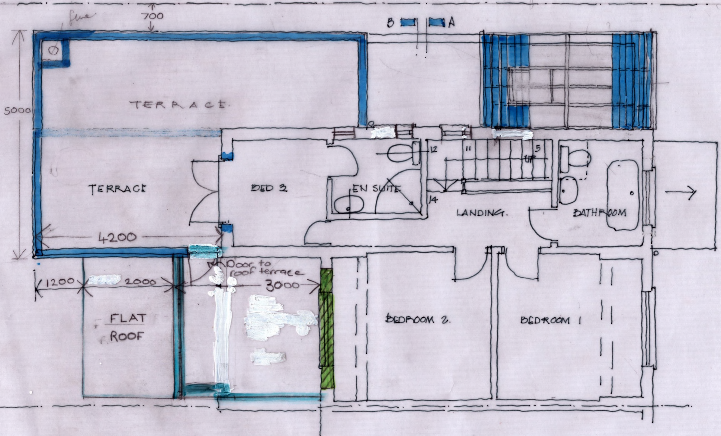
PROPOSED FIRST FLOOR PLAN. 1:50 GROUND FLOOR SIDE AND REAR EXTENSION AT 75 GARSTANG ROAD EAST. for JANE FOX.
