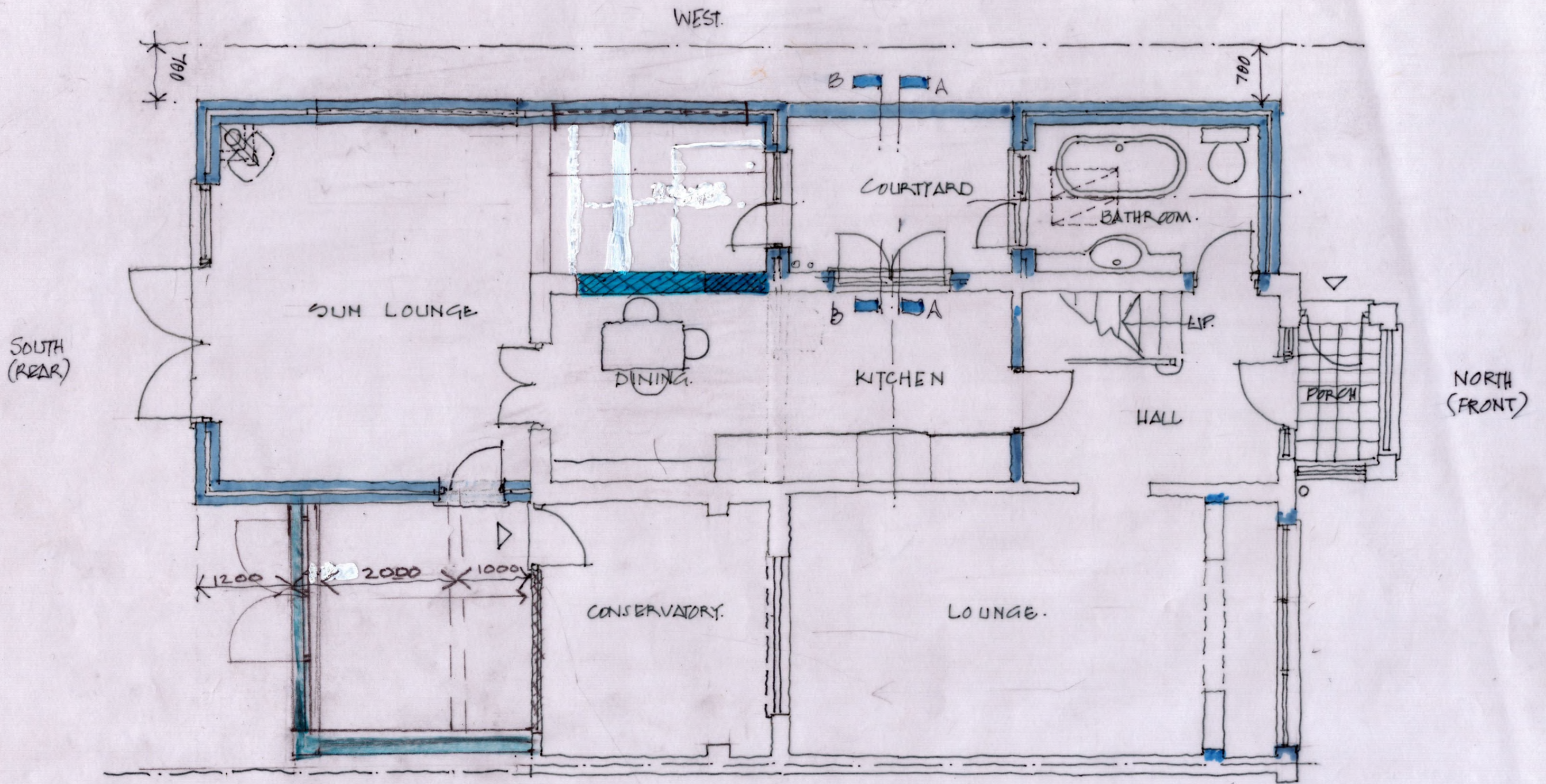
PROPOSED GROUND FLOOR PLAN 1:50. GROUND FLOOR SIDE AND REAR EXTENSION AT 75 GARSTANG ROAD EAST FOR JANE FOX.
