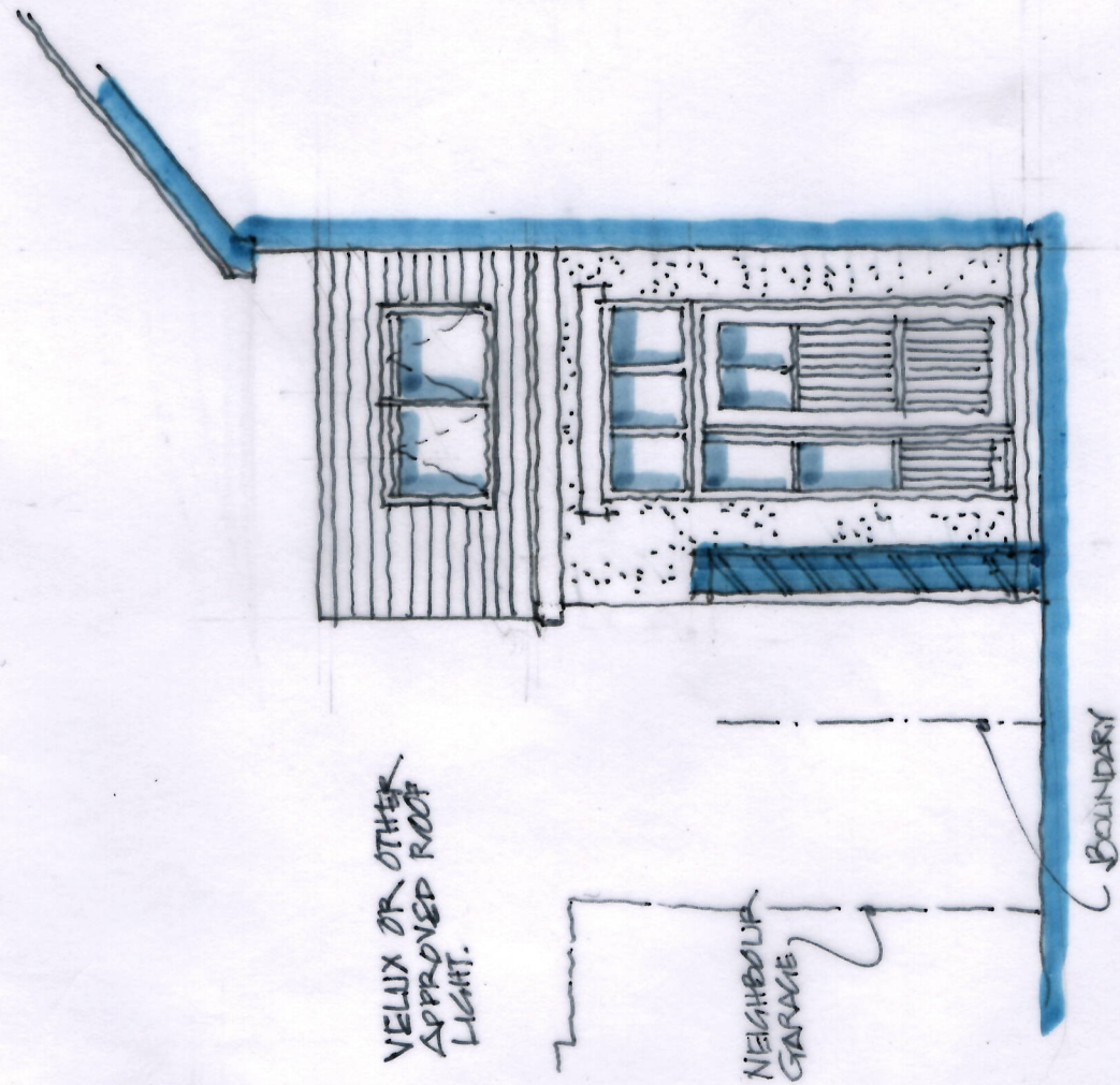
SECTION A-A 1:50 SECTIONS AT 79 GARSTANG ROAD EAST FOR JANE FOX.
