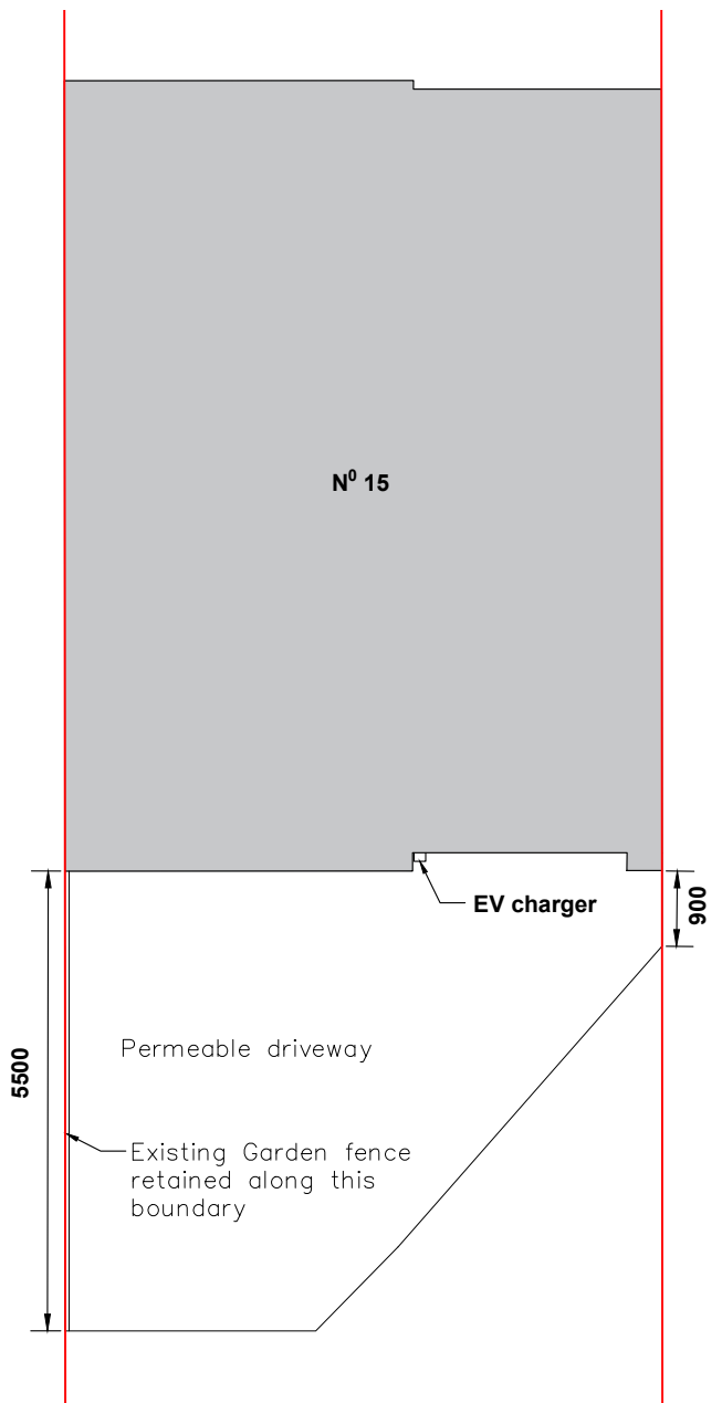
PROPOSED LAYOUT PLAN
