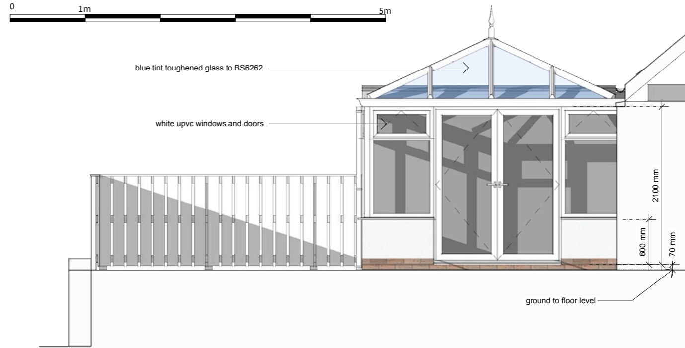
P :: PROPOSED SIDE ELEVATION
