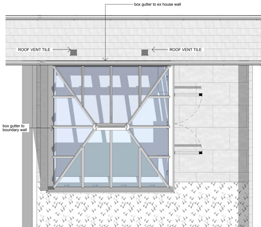
P :: PROPOSED ROOF PLAN
