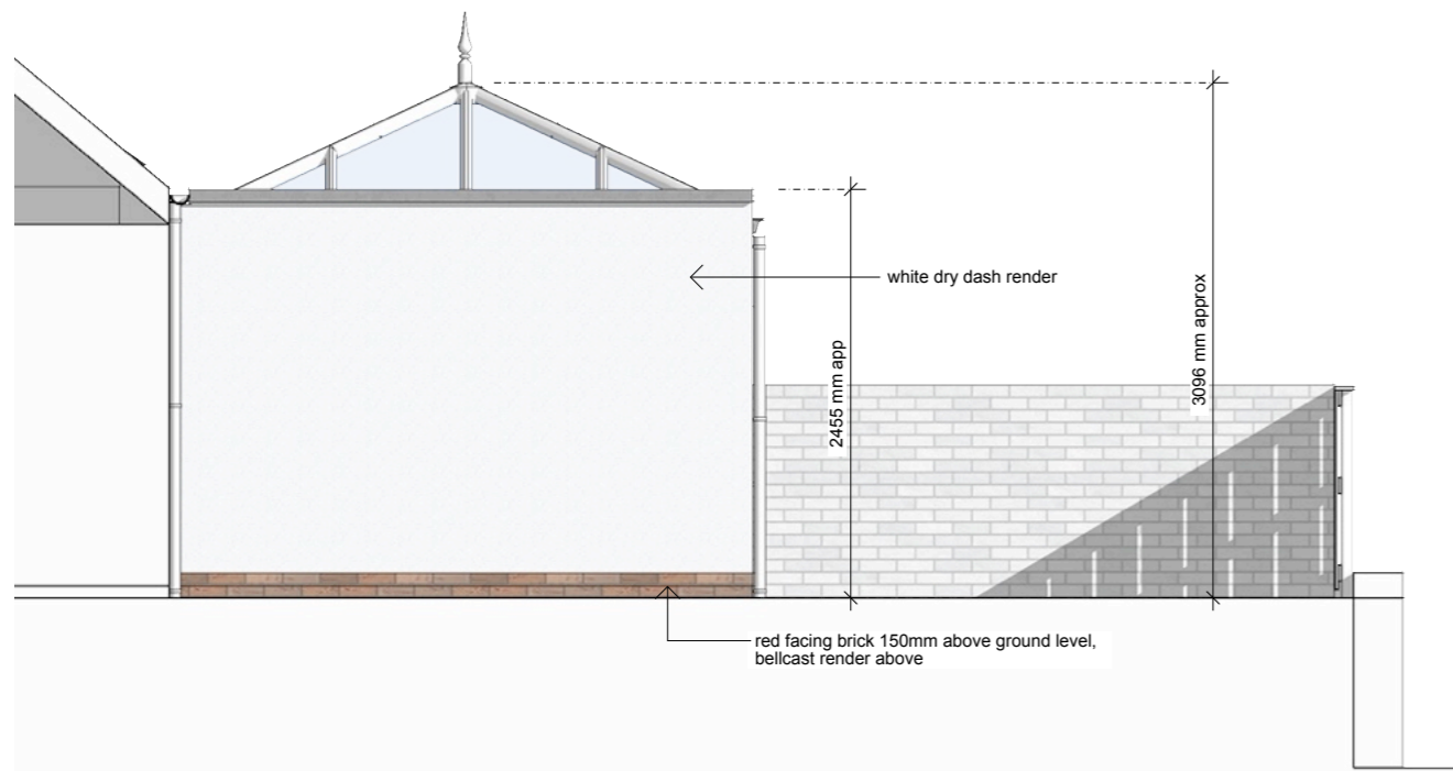
P :: PROPOSED SIDE ELEVATION
