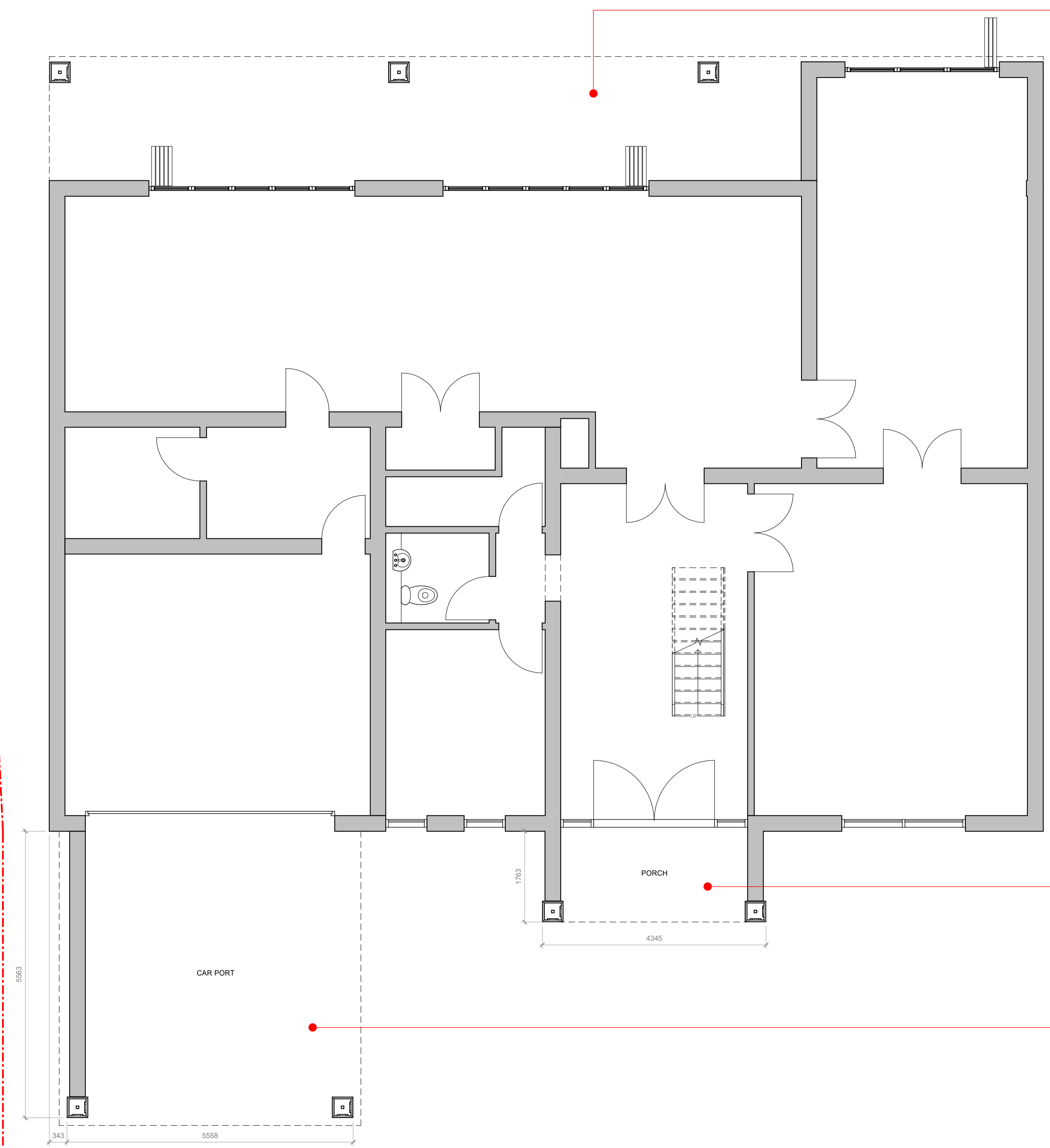
1 PROPOSED GROUND FLOOR PLAN 1 : 50
