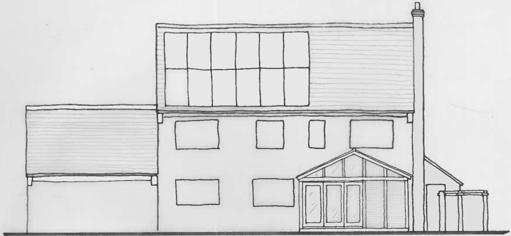
PROPOSED SOUTH EAST ELEVATION. GARDEN ROOM.
