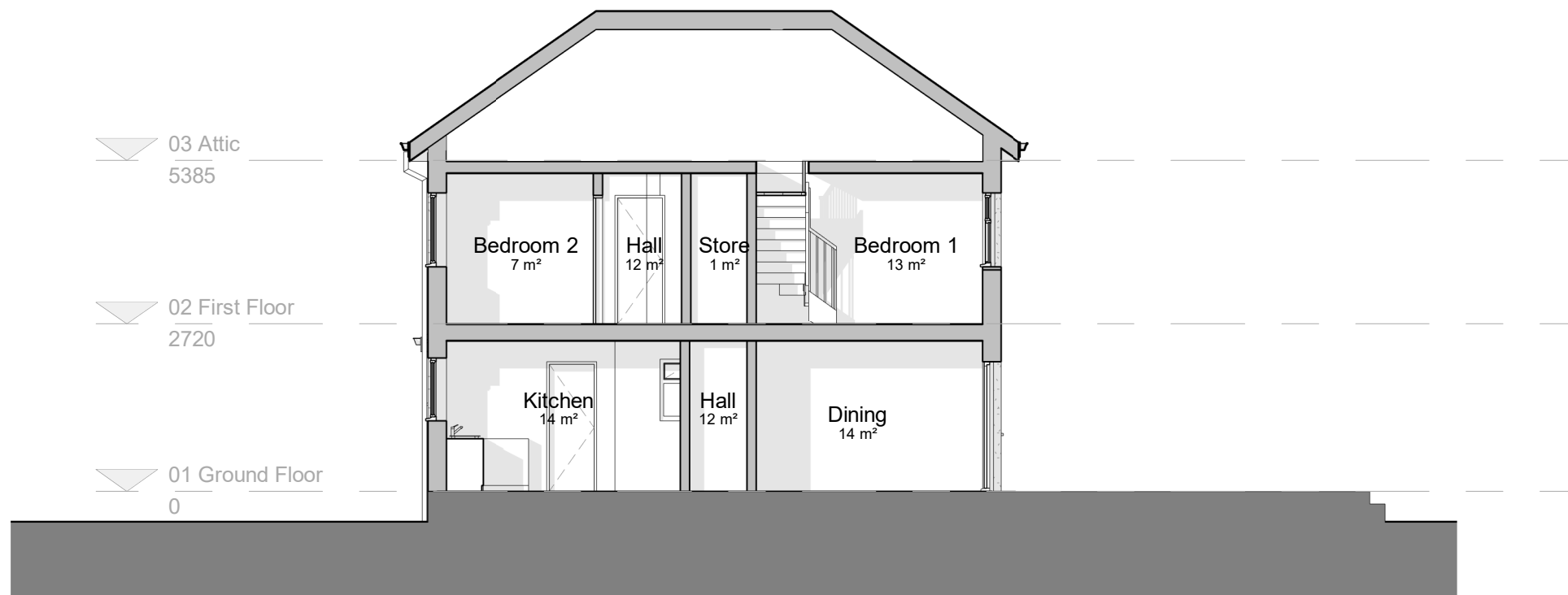
Section A-A Existing
