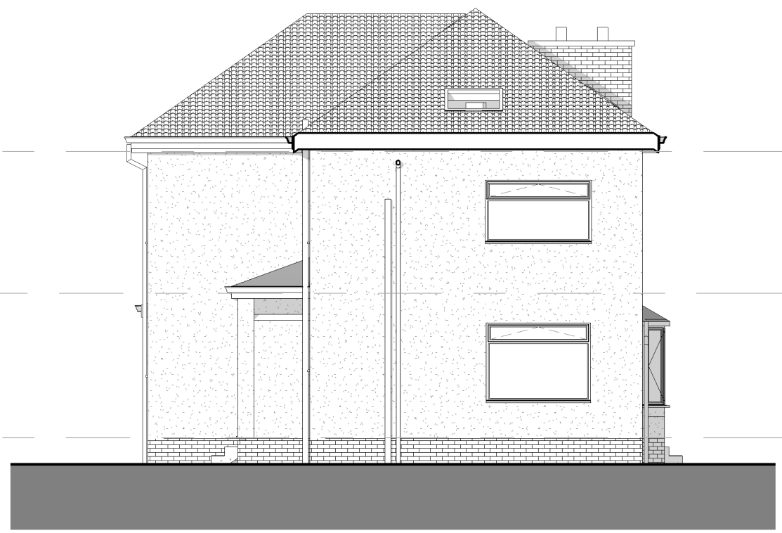
GABLE ELEVATION
