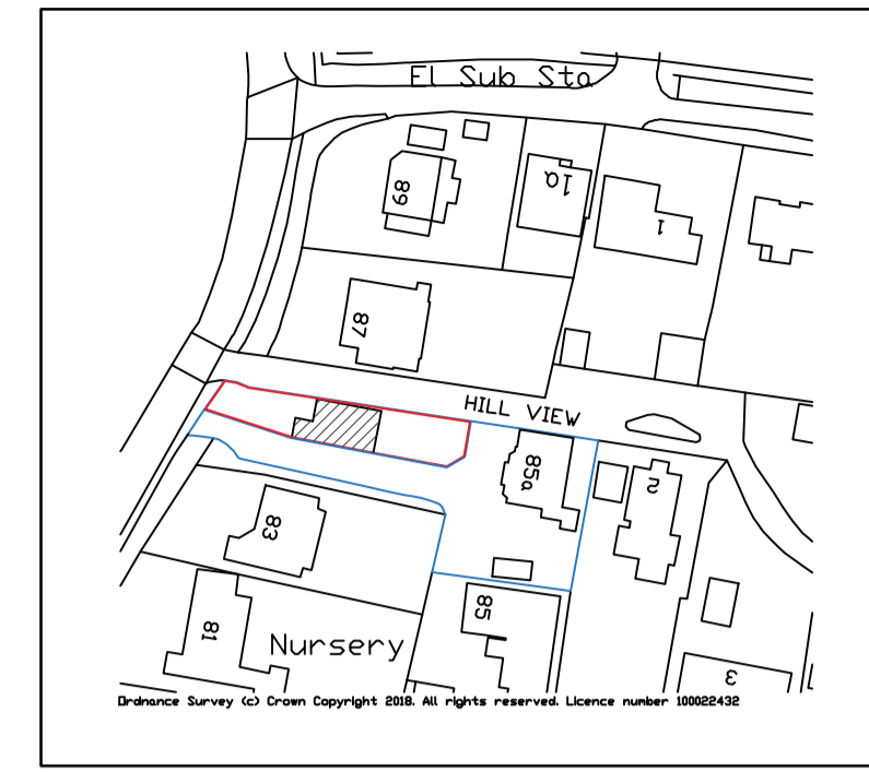
SITE LOCATION PLAN AS PROPOSED 1:1250
