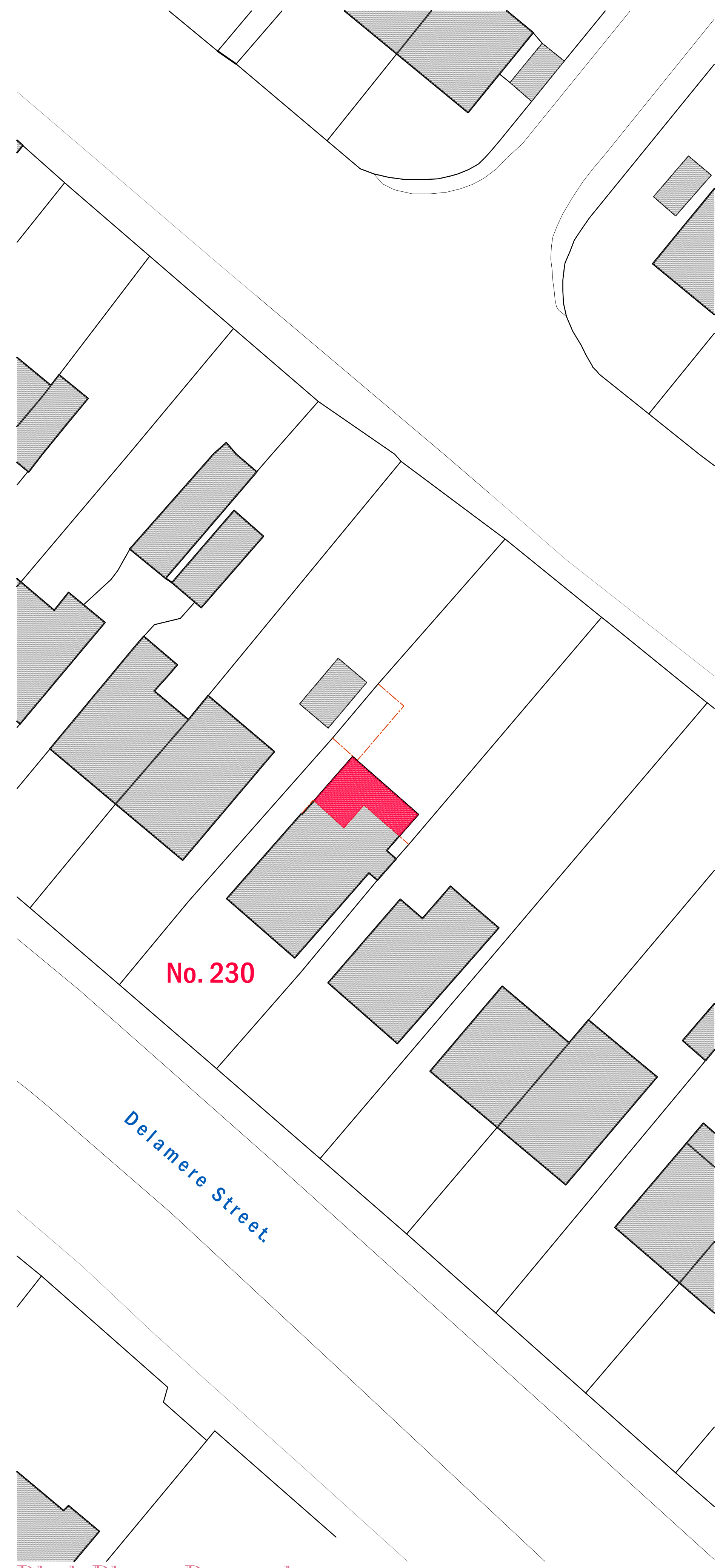
Block Plan as Proposed. Scale 1:200.
