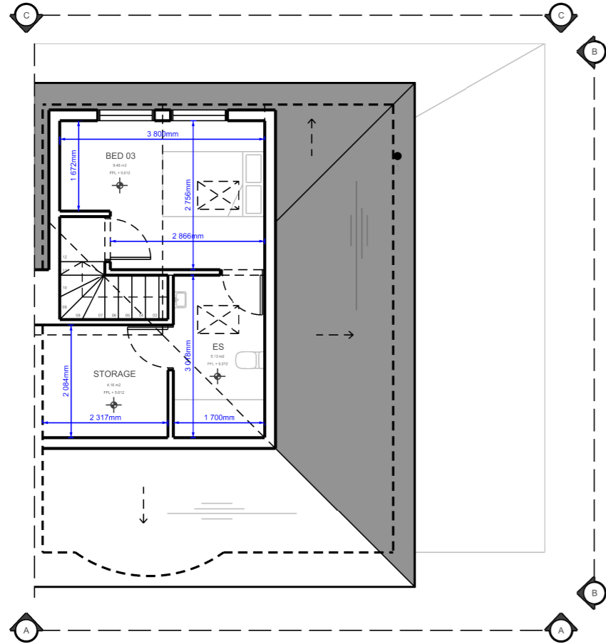
02 LOFT PLAN [PROPOSED] GIFA - 19.80
