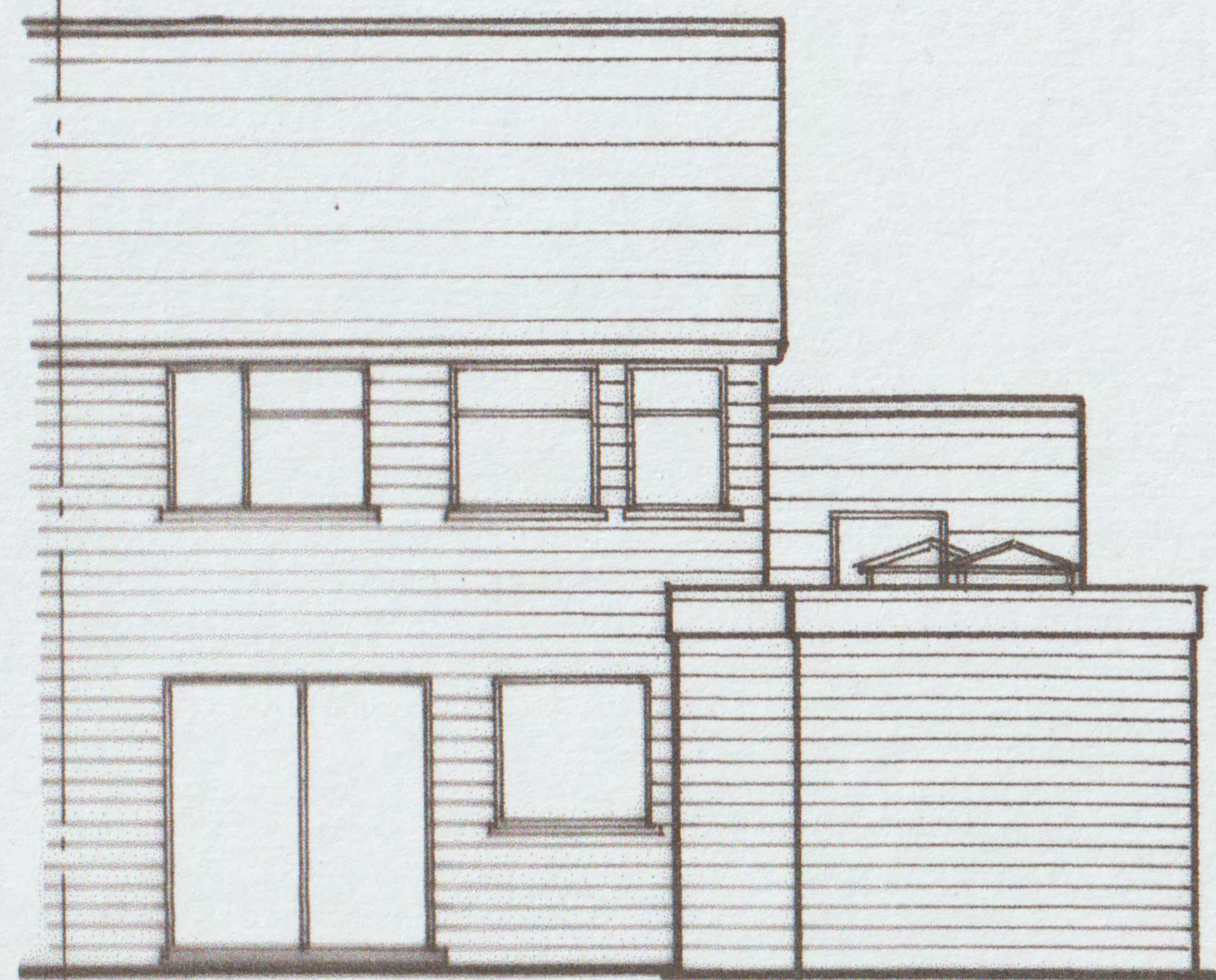
PROPOSED REAR ELEVATION
