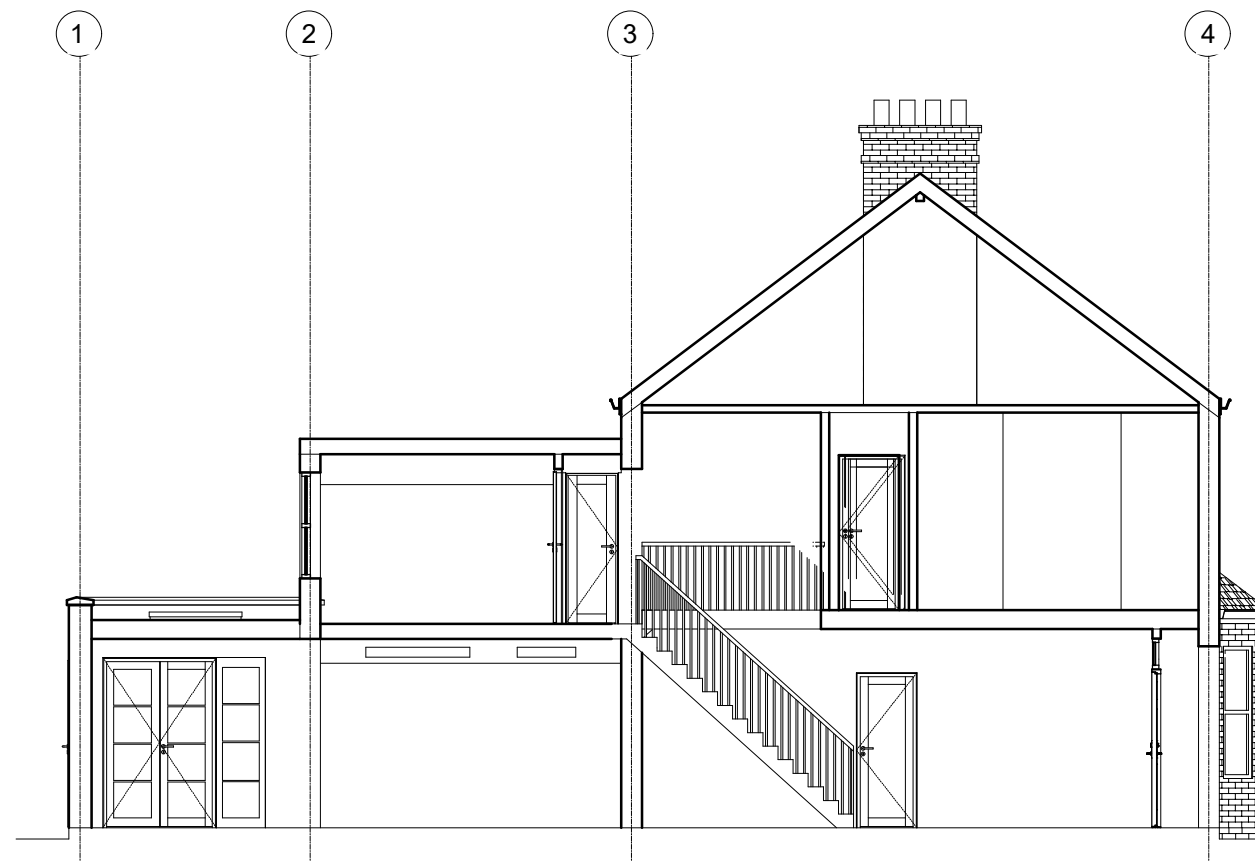
EXISTING SECTION
