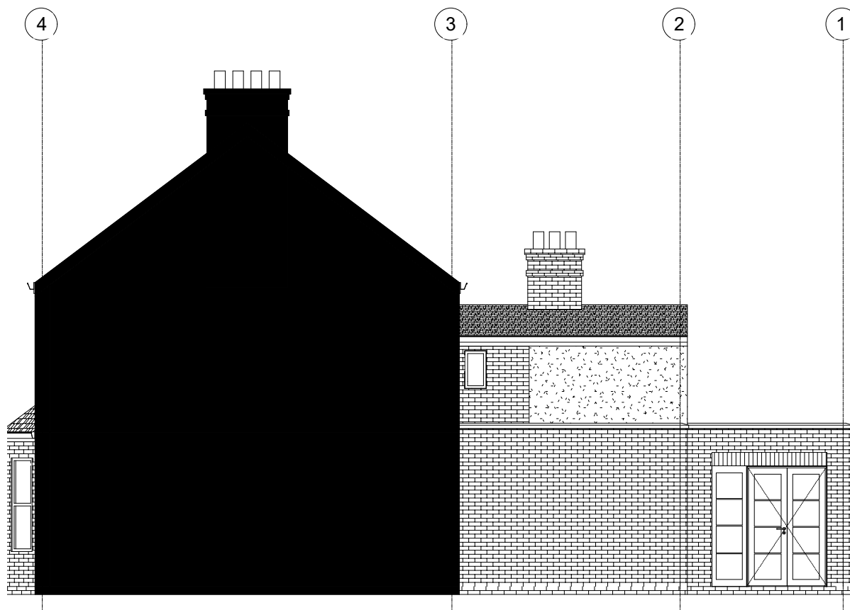
EXISTING RIGHT SIDE ELEVATION
