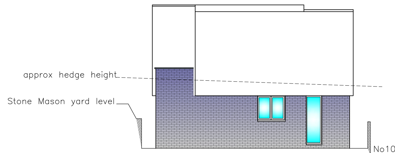
Proposed Side Elevation 1:100 (Option 1 - West)
