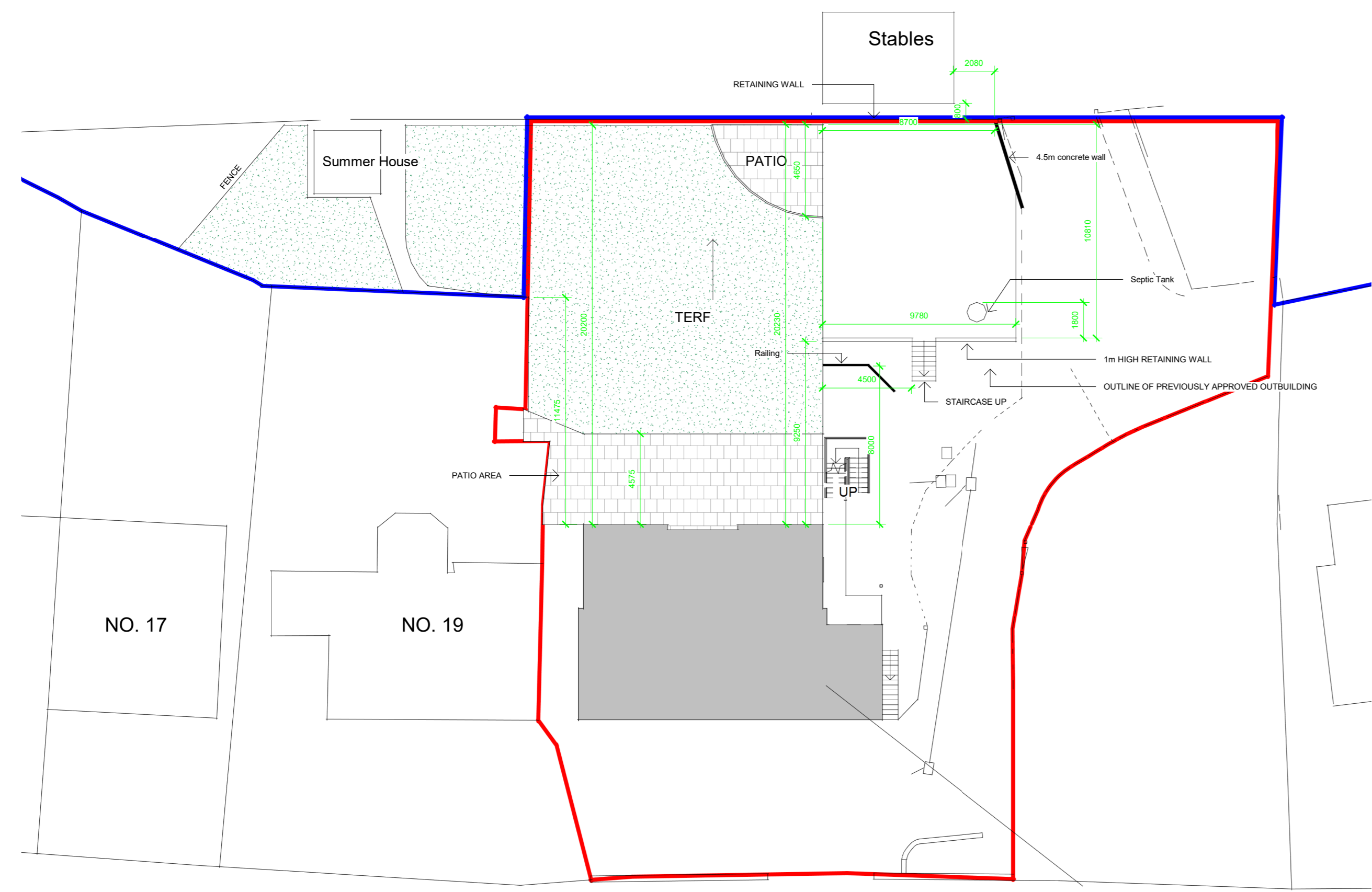
1 Site Block Plan - Existing (c) 1 : 200
