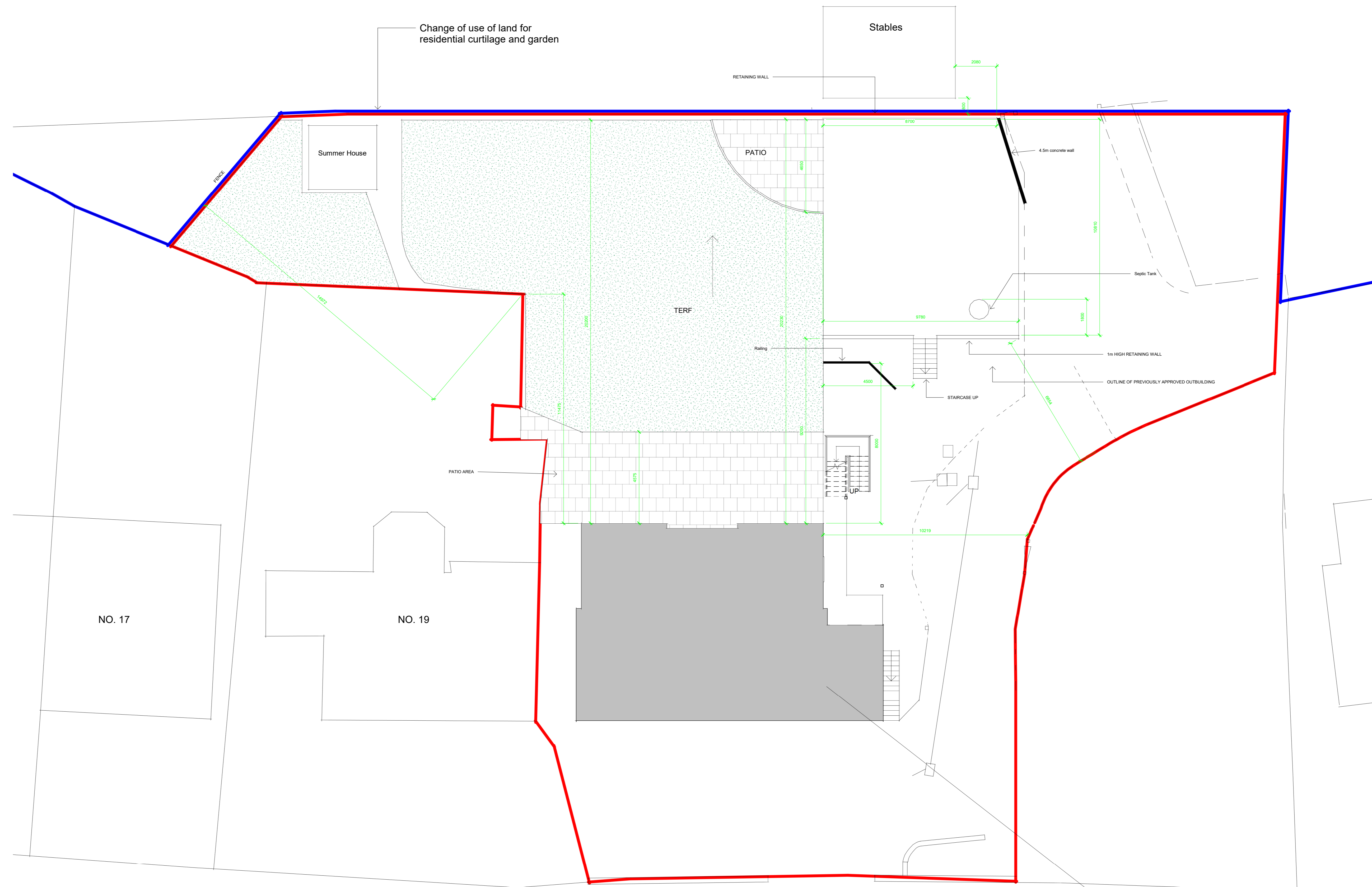
2 Site Block Plan - Proposed (c) 1 : 100
