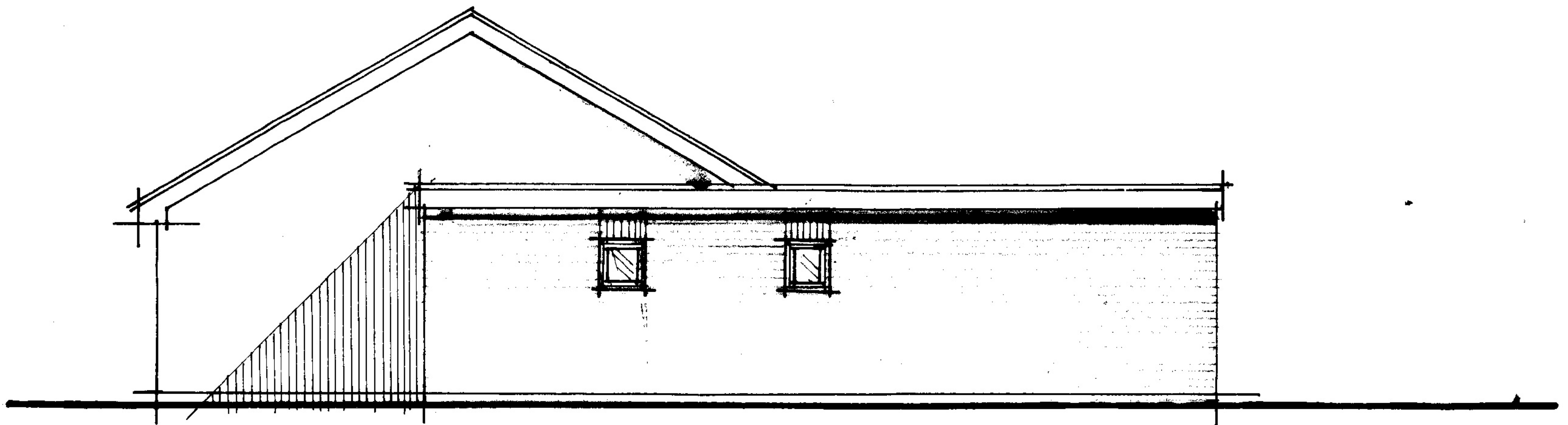
EAST ELEVATION.
