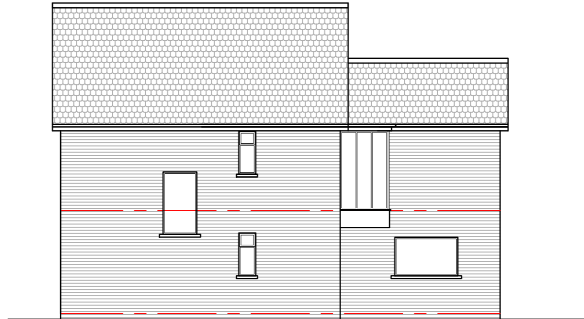
EXISTING SIDE ELEVATION [facing No. 14]
