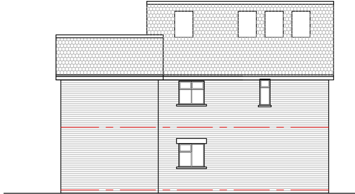
EXISTING SIDE ELEVATION [facing No. 18]
