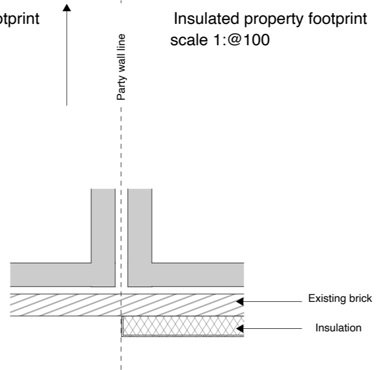
Party wall plan detail scale 1:@20
